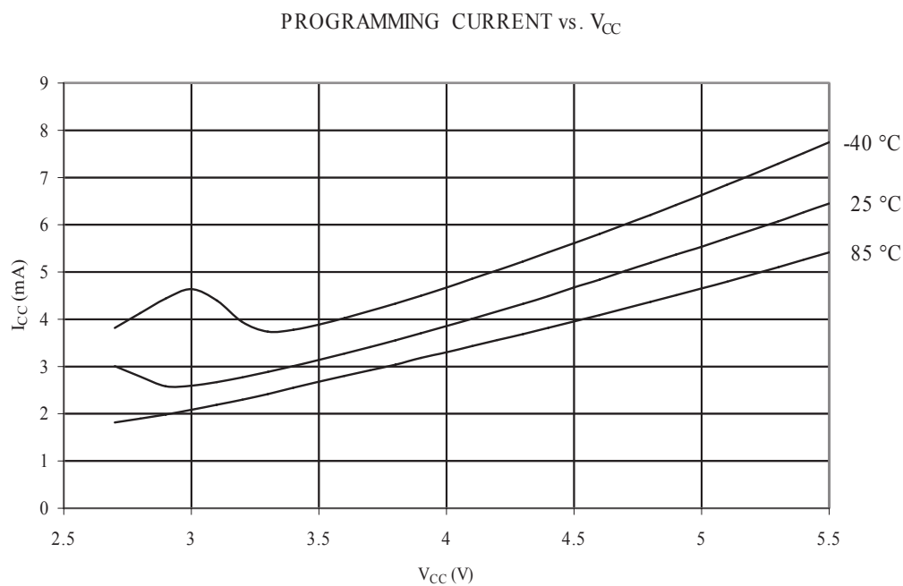
Figure 33-49 Programming Current vs. V_{CC}
