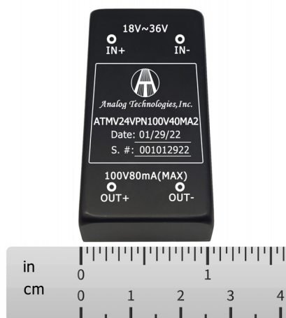
Figure 1. Top View of ATMV24VPN100V40MA2
