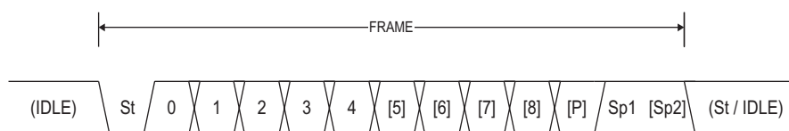
Figure 72. Frame Formats
