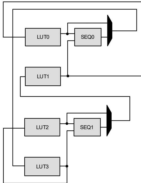
Figure 27-4. Linked LUT Input Selection
