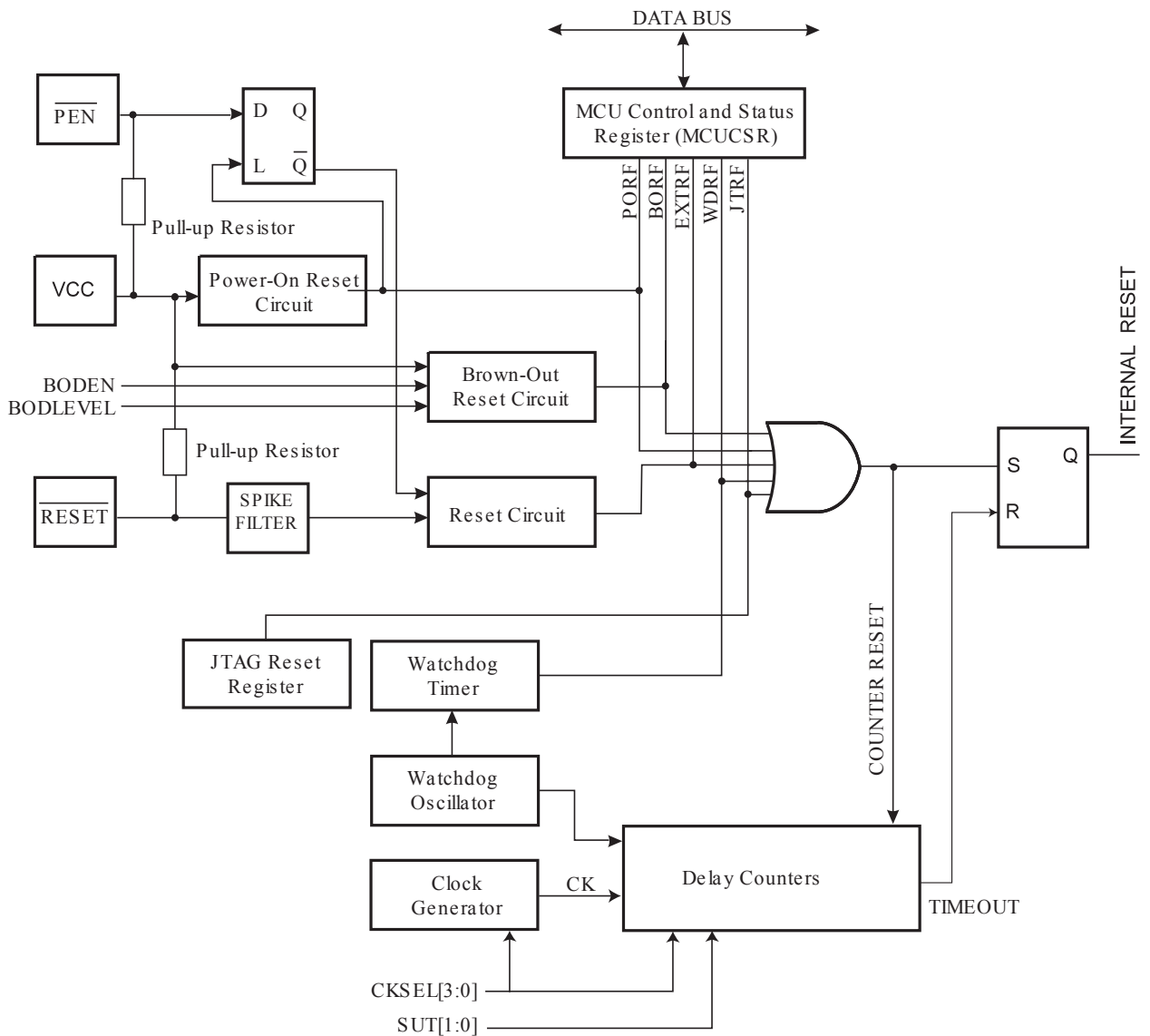
Figure 15-1 Reset Logic
