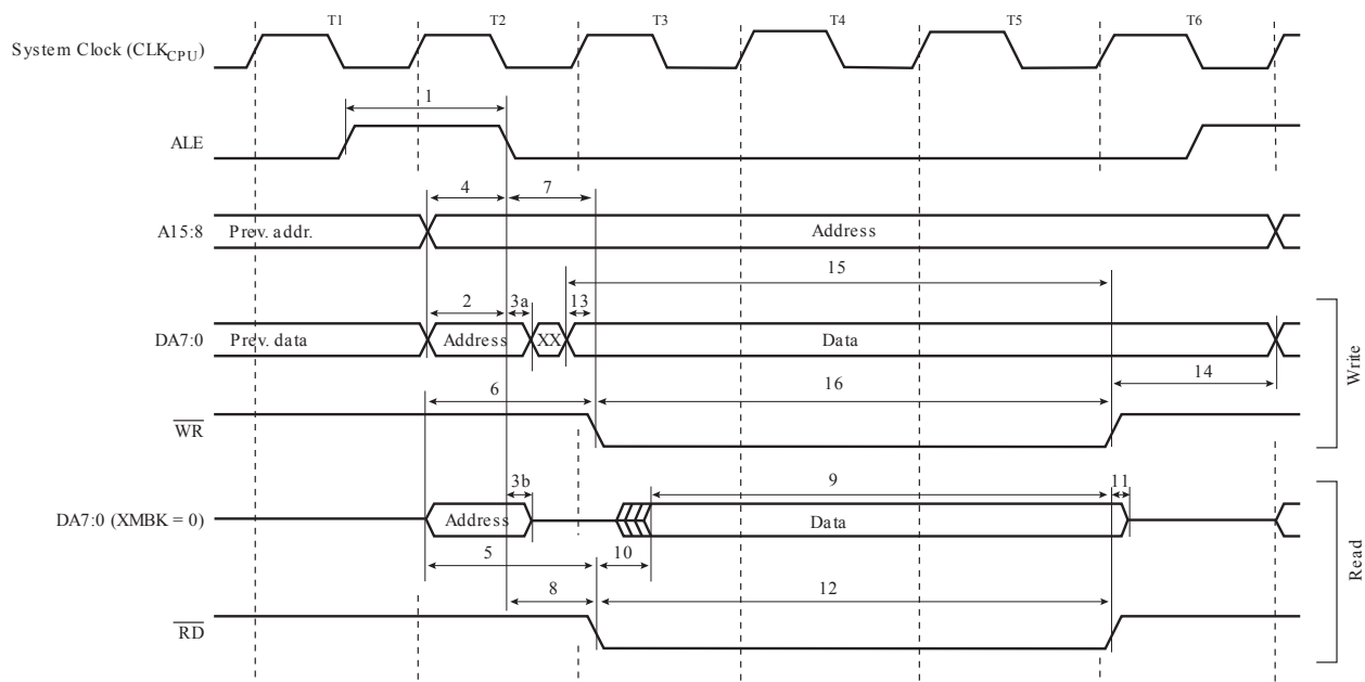
Figure 32-10 External Memory Timing (SRWn1 = 1, SRWn0 = 0)
