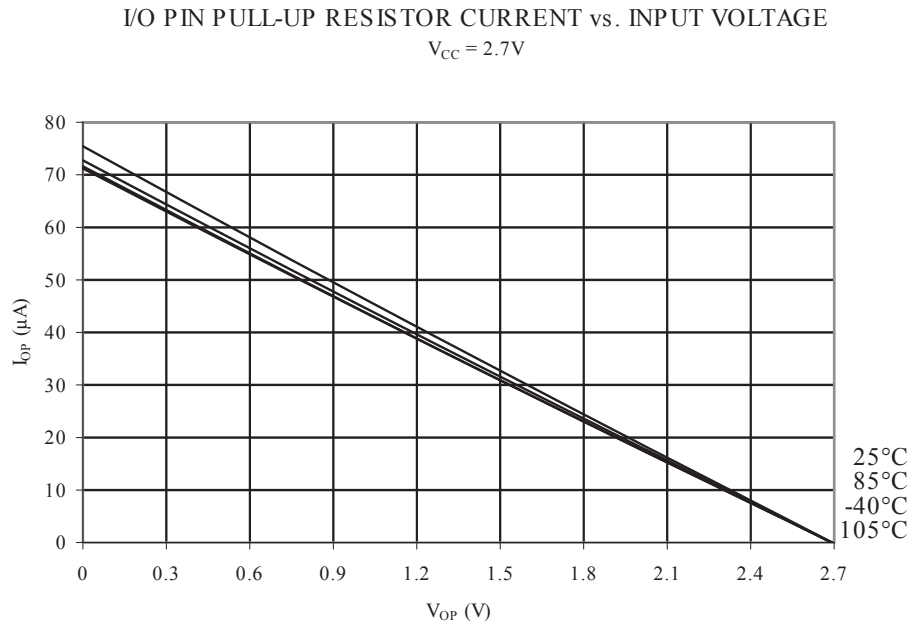
Figure 35-16 I/O Pin Pull-up Resistor Current vs. Input Voltage (VCC = 2.7V)
