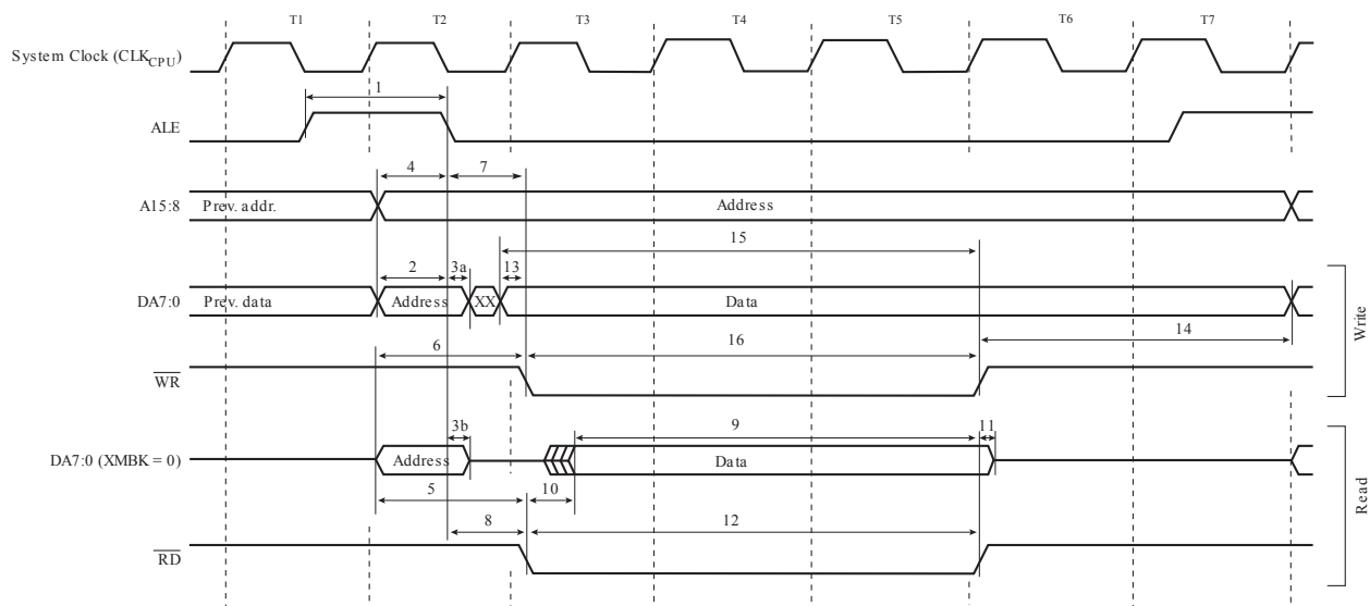
Figure 32-11 External Memory Timing (SRWn1 = 1, SRWn0 = 1)
