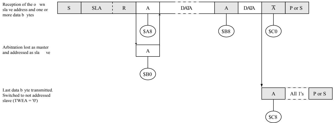
Figure 26-18 Formats and States in the Slave Transmitter Mode
