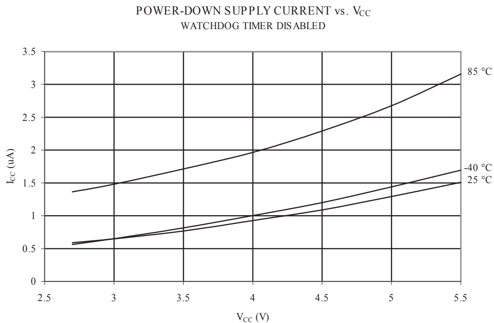
Figure 34-15 Power-Down Supply Current vs. V_{CC} (Watchdog Timer Disabled)
