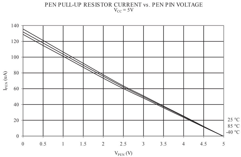
Figure 34-24 PEN Pull-up Resistor Current vs. PEN Pin Voltage ( V_{CC} = 5V )
