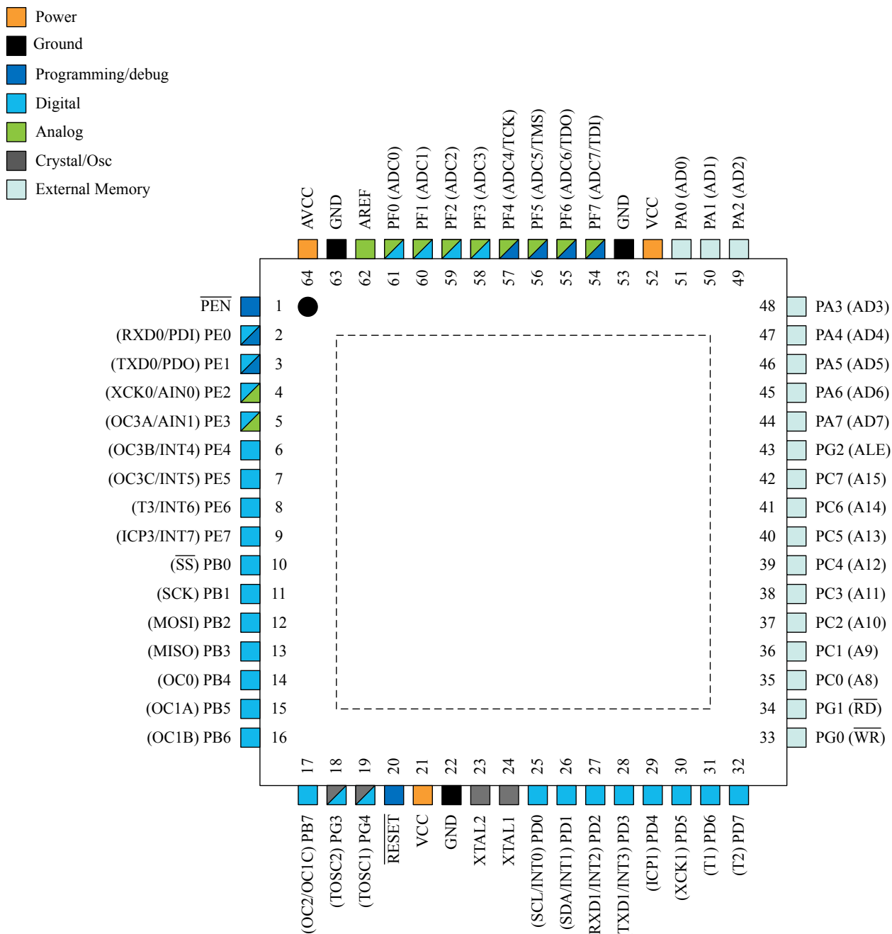
Figure 6-1 Pinout ATmega64A
