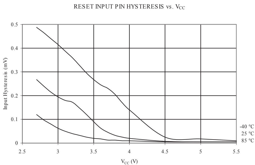
Figure 34-35 Reset Input Pin Hysteresis vs. V_{CC}
