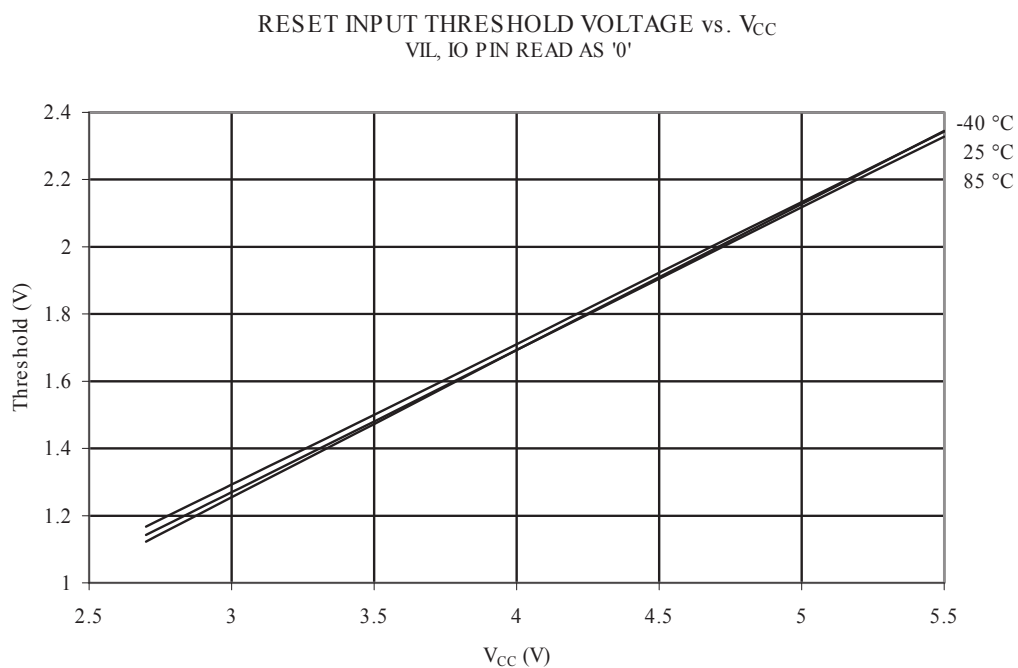
Figure 34-34 Reset Input Threshold Voltage vs. V_{CC} (VIL, Reset Pin Read as '0')
