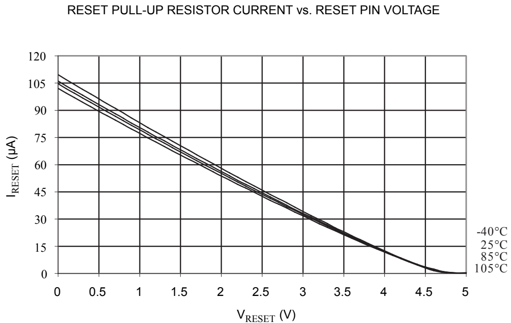
Figure 35-17 Reset Pull-up Resistor Current vs. Reset Pin Voltage (VCC = 5V)
