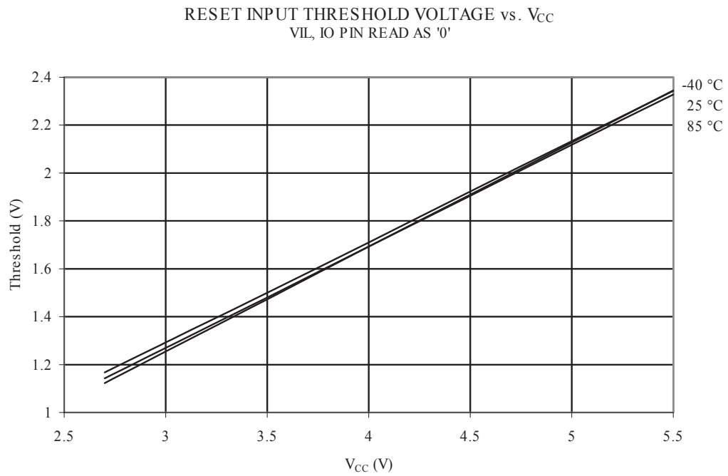
Figure 34-34 Reset Input Threshold Voltage vs. V_{CC} (VIL, Reset Pin Read as '0')
