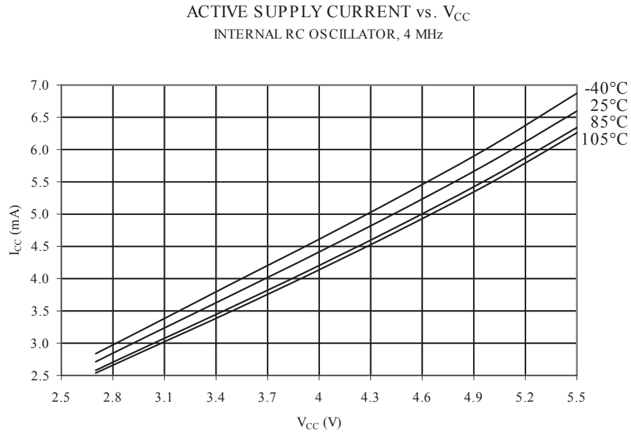
Figure 35-4 Active Supply Current vs. V_{CC} (Internal RC Oscillator, 4MHz)
