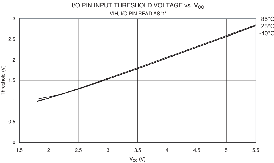
Pin Thresholds and hysteresis Figure 174. I/O Pin Input Threshold Voltage vs. V_{CC} ( V_{IH} , I/O Pin Read as “1”)
