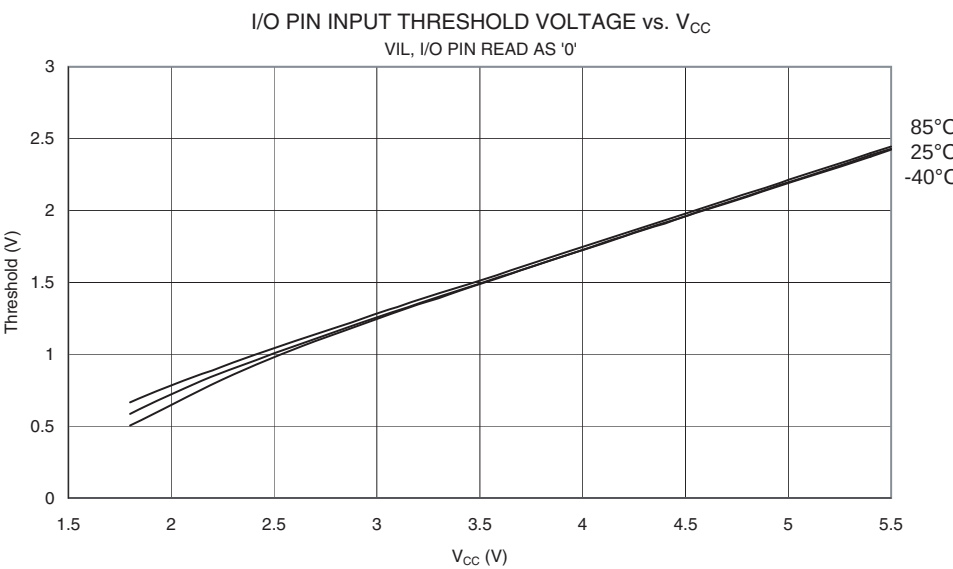
Figure 175. I/O Pin Input Threshold Voltage vs. V_{CC} ( V_{IL} , I/O Pin Read as “0”)
