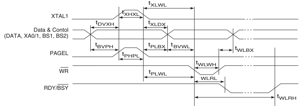
Figure 118. Parallel Programming Timing, Loading Sequence with Timing Requirements (1)
