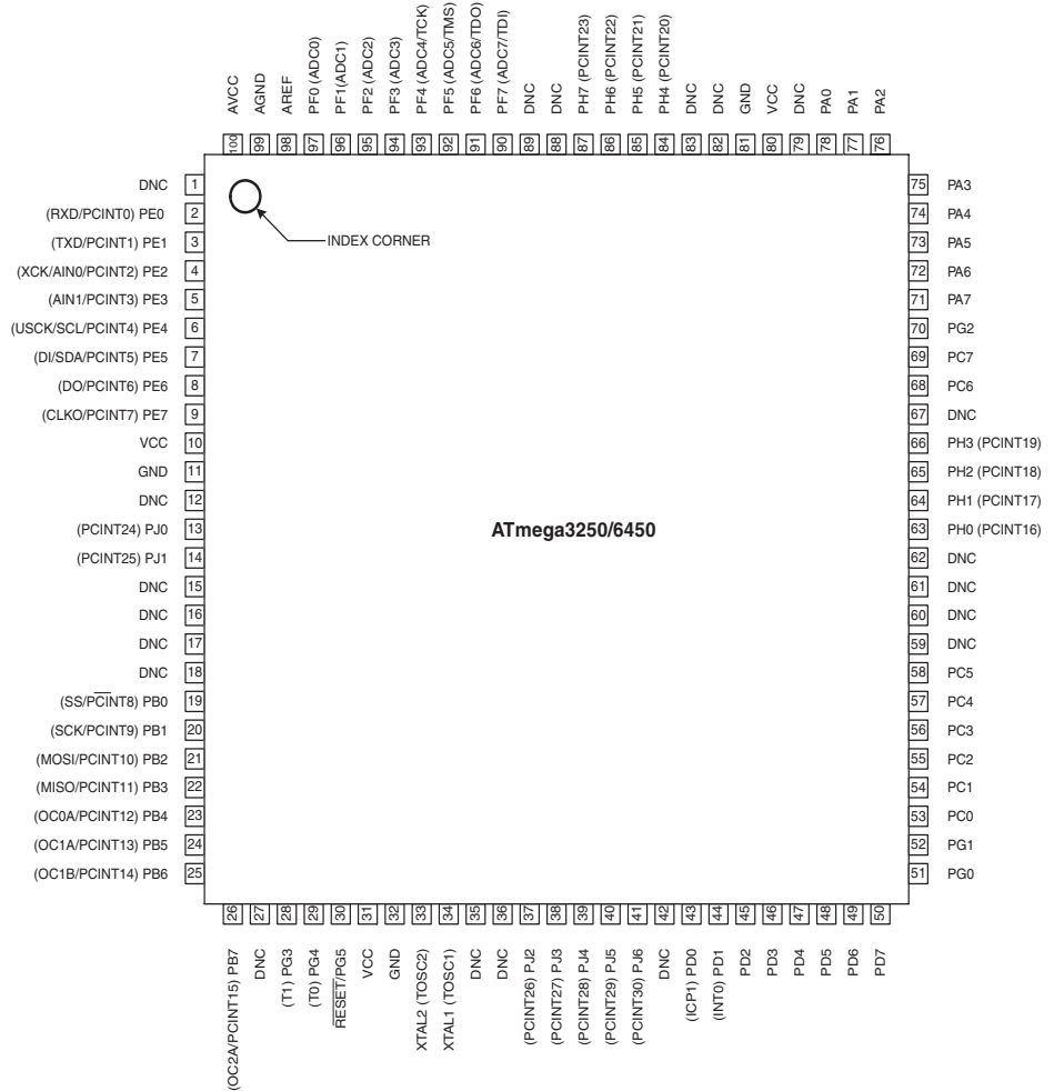
Figure 1. Pinout ATmega3250/6450
