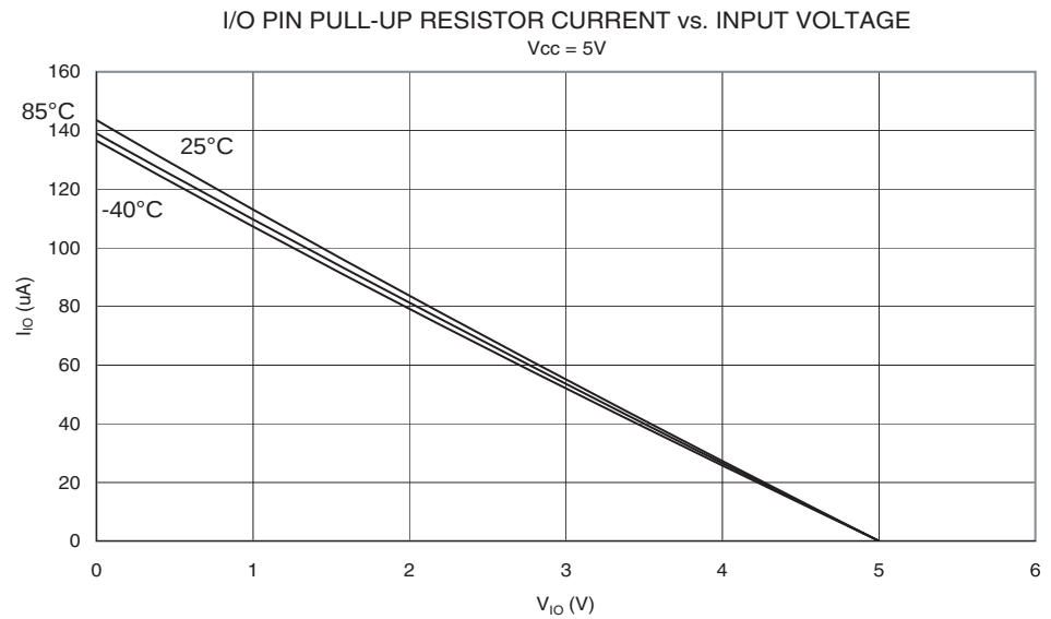
Figure 148. I/O Pin Pull-up Resistor Current vs. Input Voltage ( V_{CC} = 5V )
