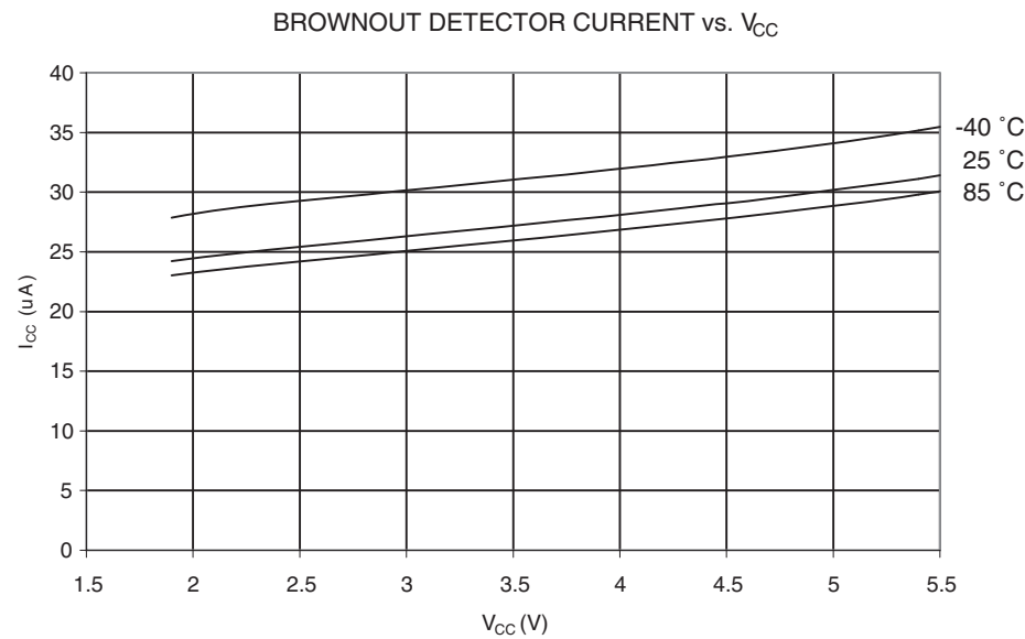
Figure 182. Brownout Detector Current vs. V_{CC}
