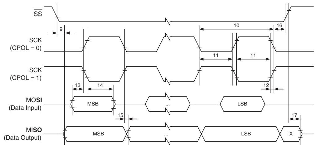
Figure 133. SPI Interface Timing Requirements (Slave Mode)
