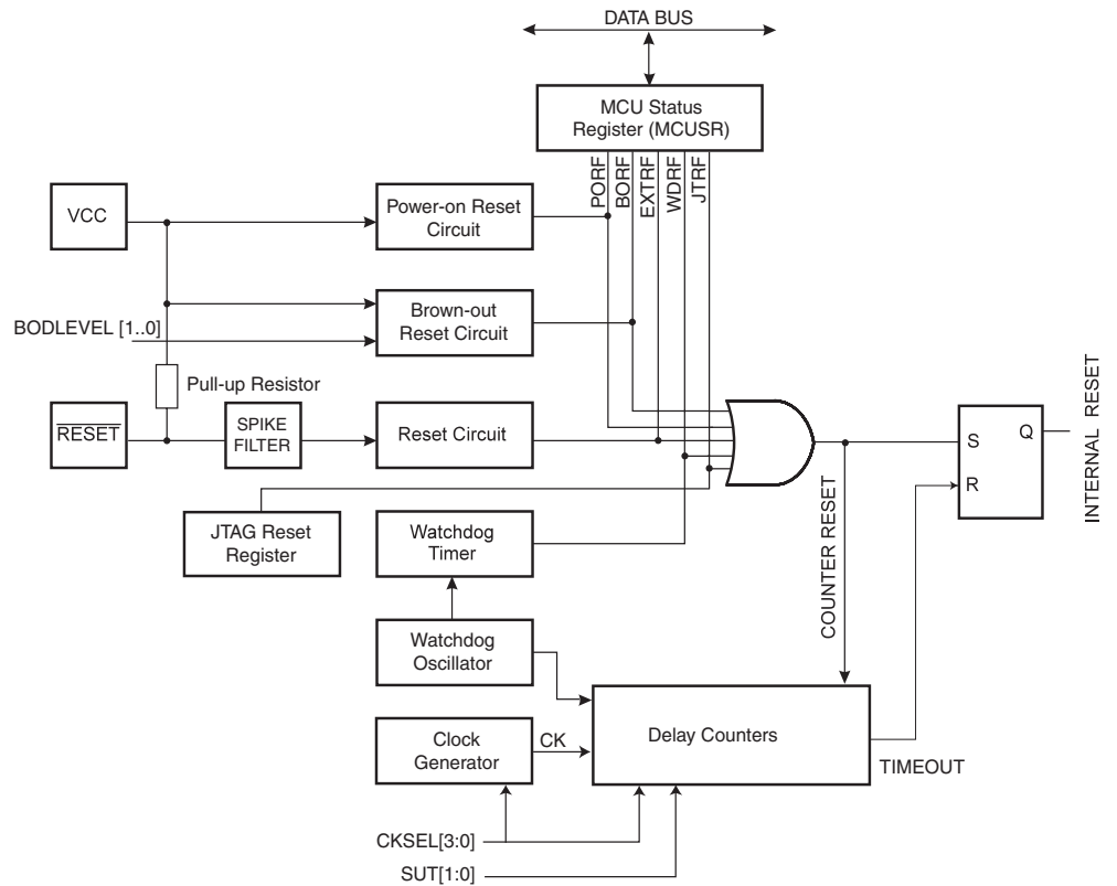
Figure 15. Reset Logic
