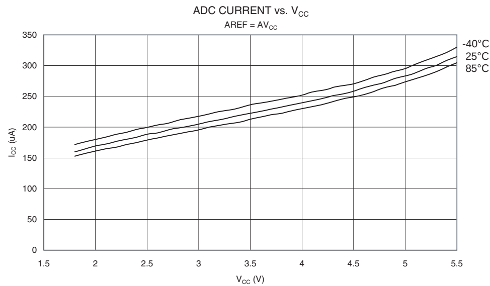
Figure 183. ADC Current vs. V_{CC} (AREF = AVCC)
