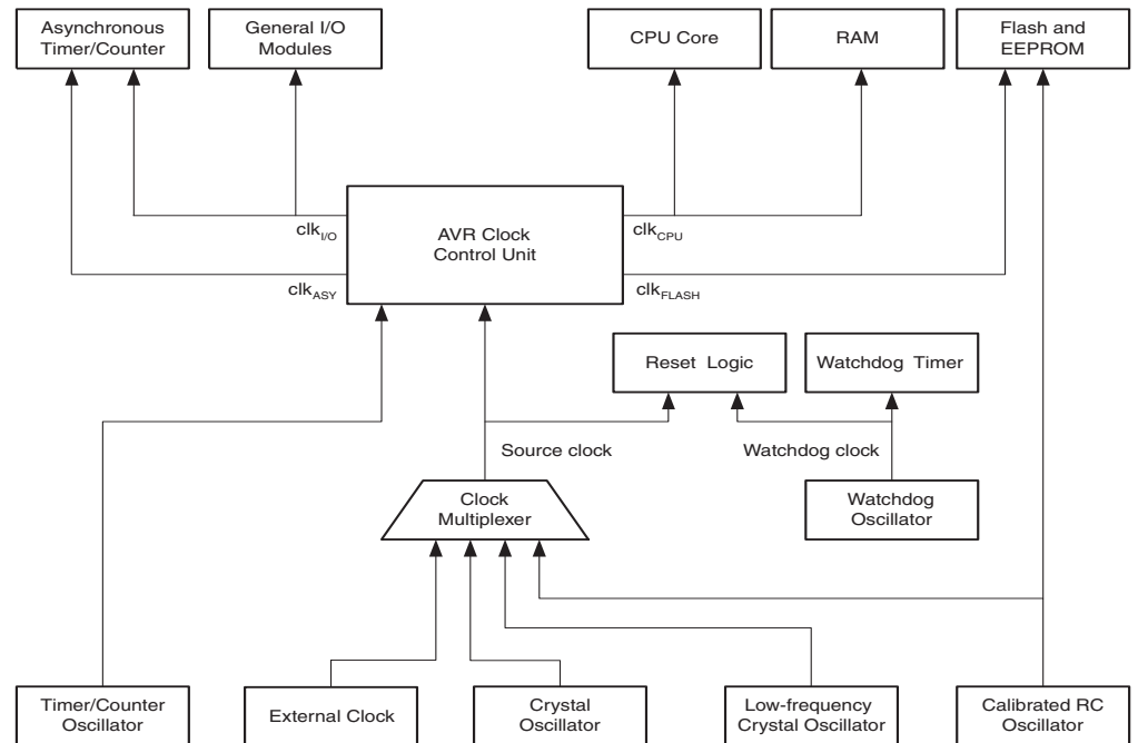
Figure 12. Clock Distribution
