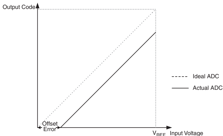
Figure 93. Offset Error
