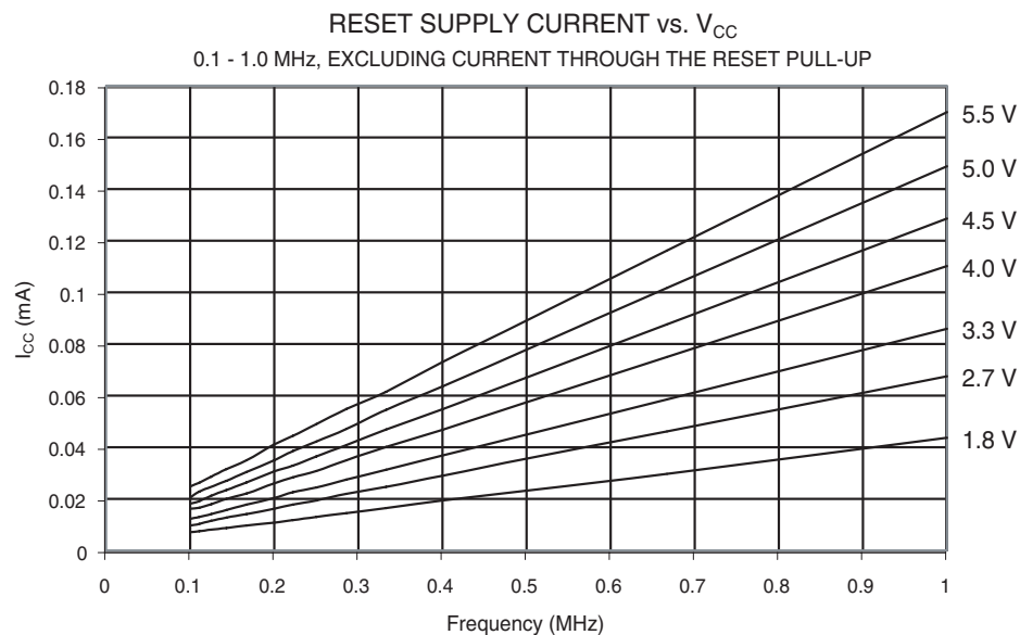
Figure 29-48. Reset Supply Current vs. V_{CC} (0.1 - 1.0 MHz, Excluding Current through the Reset Pull-up)
