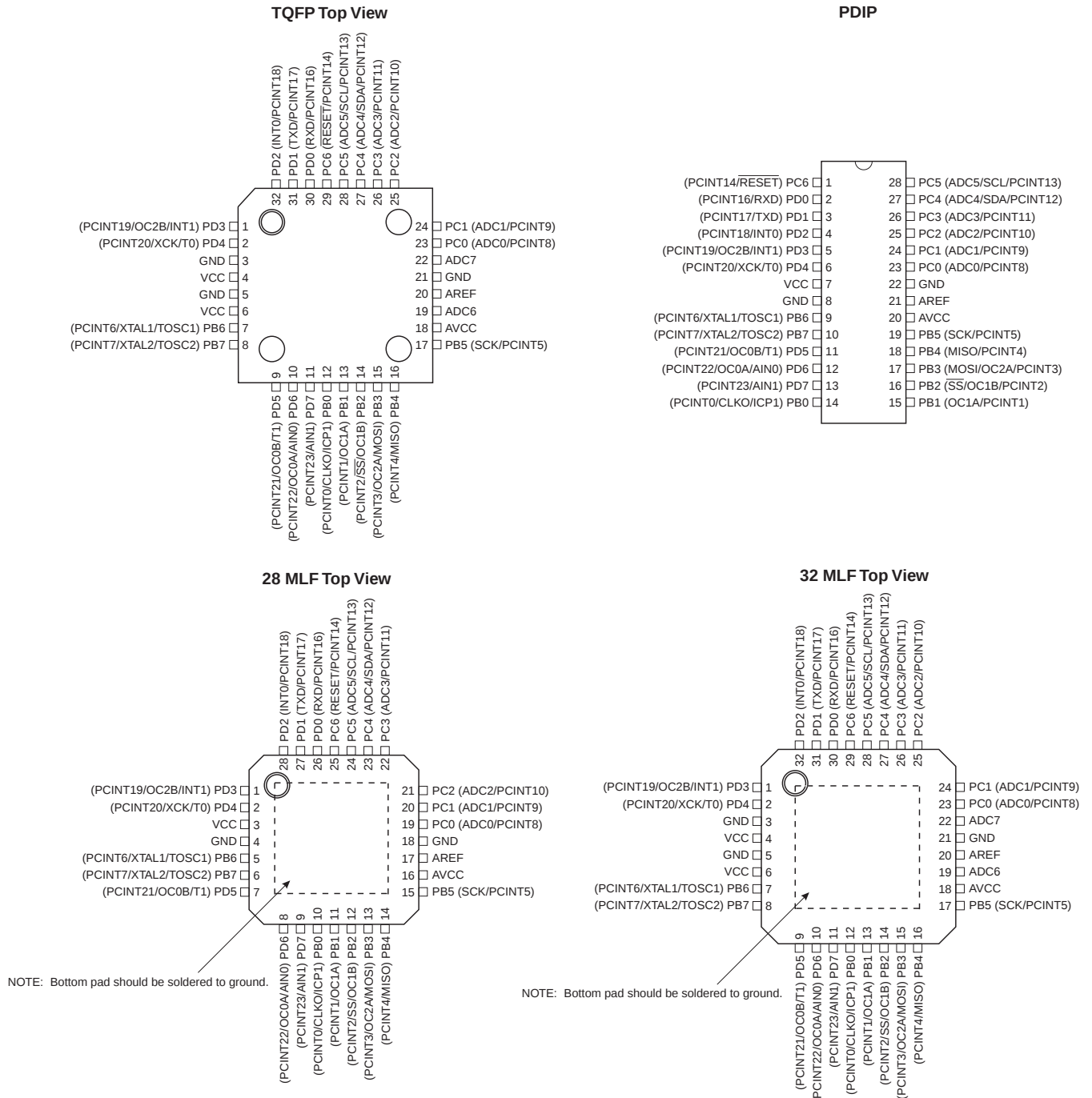
Figure 1-1. Pinout ATmega48/88/1682545M
