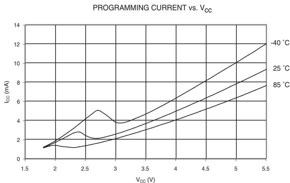
Figure 29-47. Programming Current vs. V_{CC}
