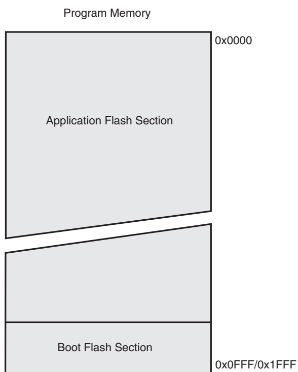
Figure 7-2. Program Memory Map, ATmega88 and ATmega168
