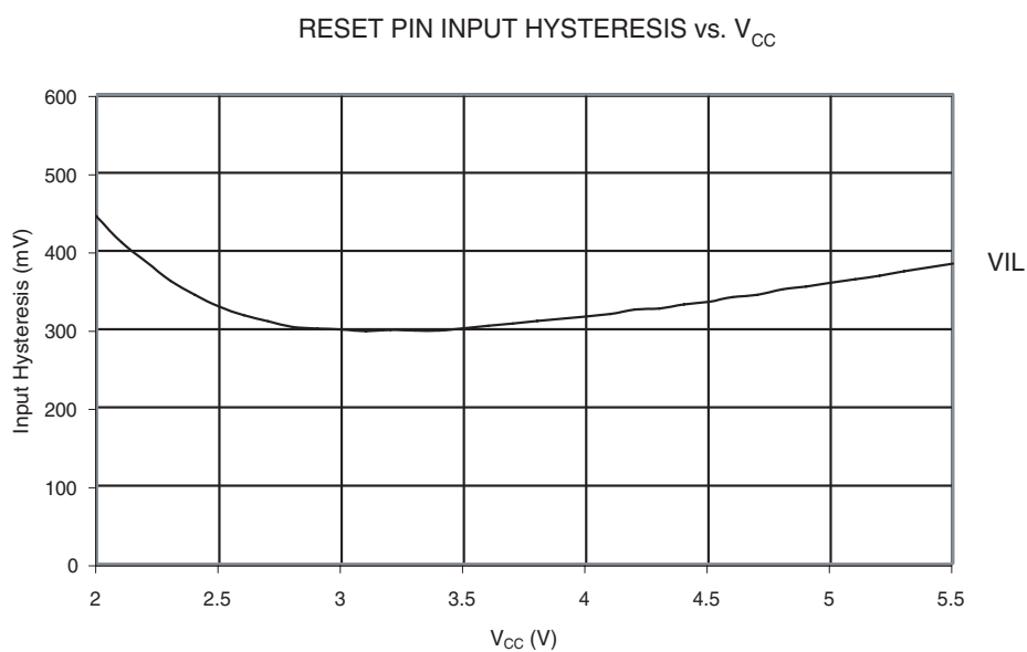
Figure 29-32. Reset Input Pin Hysteresis vs. V_{CC}
