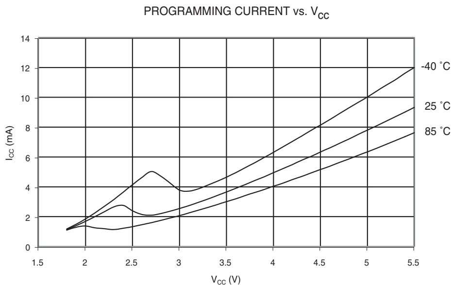
Figure 29-48. Programming Current vs. V_{CC}
