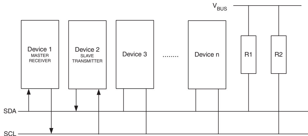
Figure 25-14. Data Transfer in Master Receiver Mode
