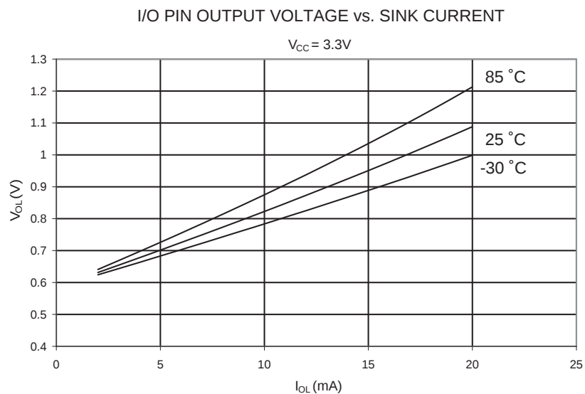
Figure 31-3. I/O Pin Putput Voltage vs. Sink Current ( V_{CC} = 3.3V )
