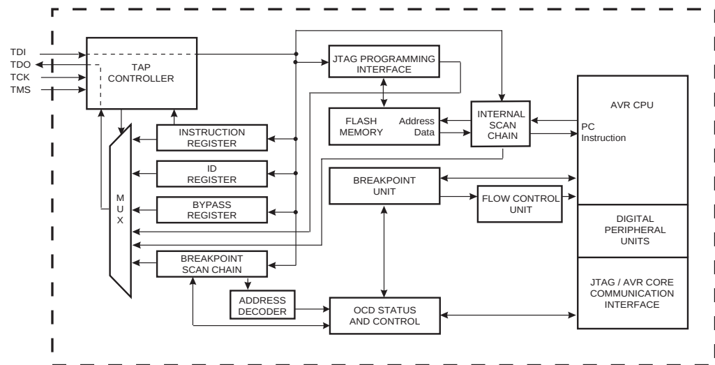
Figure 26-1. Block Diagram
