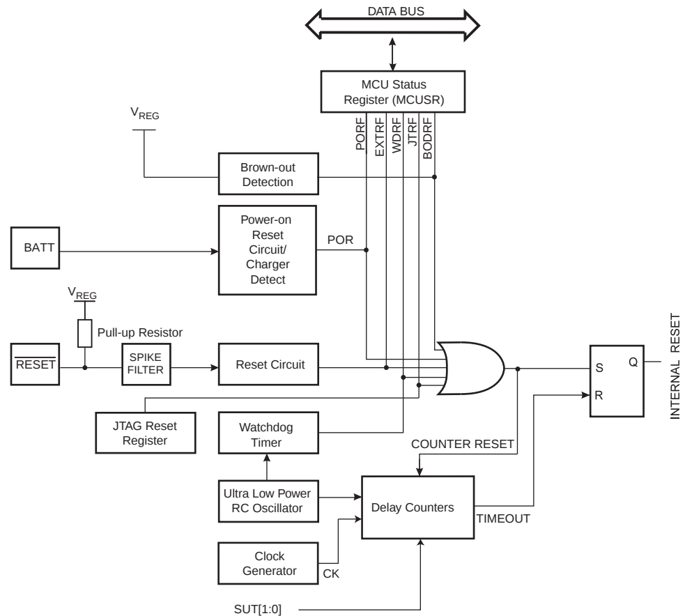
Figure 9-1. Reset Logic
