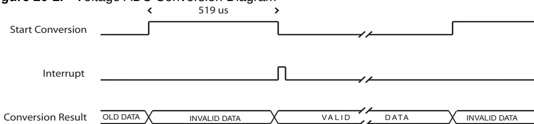
Figure 20-2. Voltage ADC Conversion Diagram
