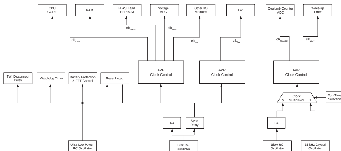
Figure 7-1. Clock Distribution
