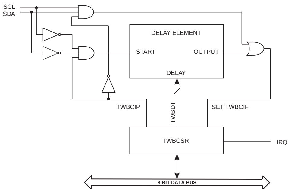
Figure 25-23. Overview of Bus Connect/Disconnect.
