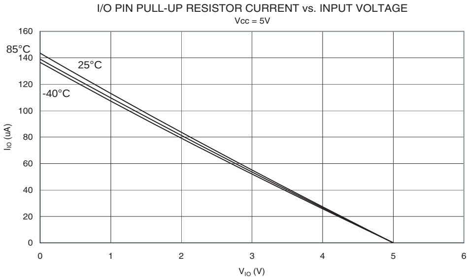
Figure 156. I/O Pin Pull-up Resistor Current vs. Input Voltage ( V_{CC} = 5V )
