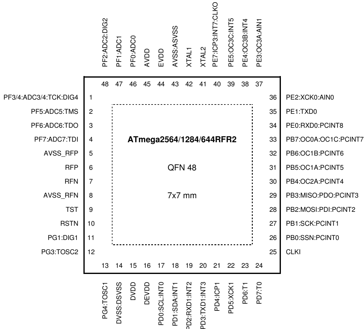
Figure 1-1. Pinout ATmega2564/1284/644RFR2
