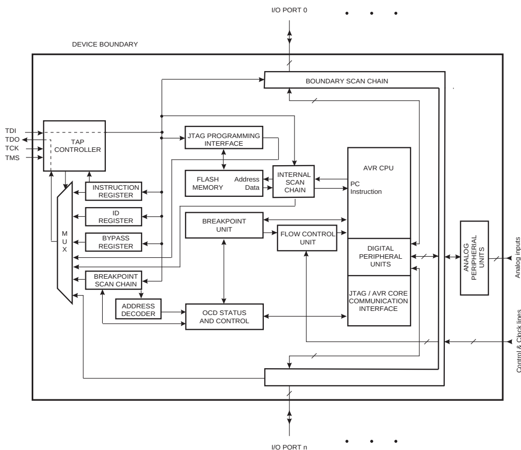
Figure 23-1. Block Diagram
