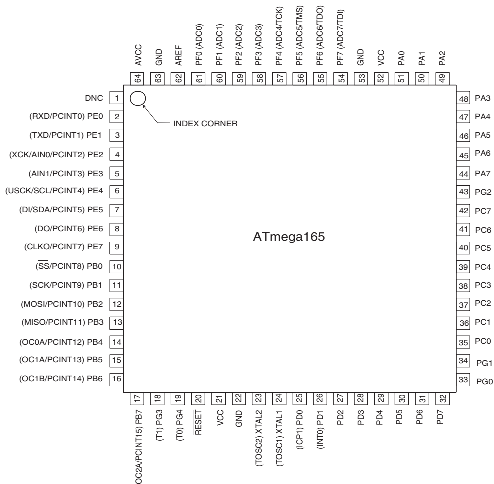
Figure 1. Pinout ATmega165
