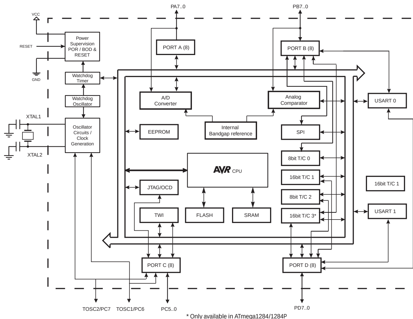
Figure 2-1. Block diagram
