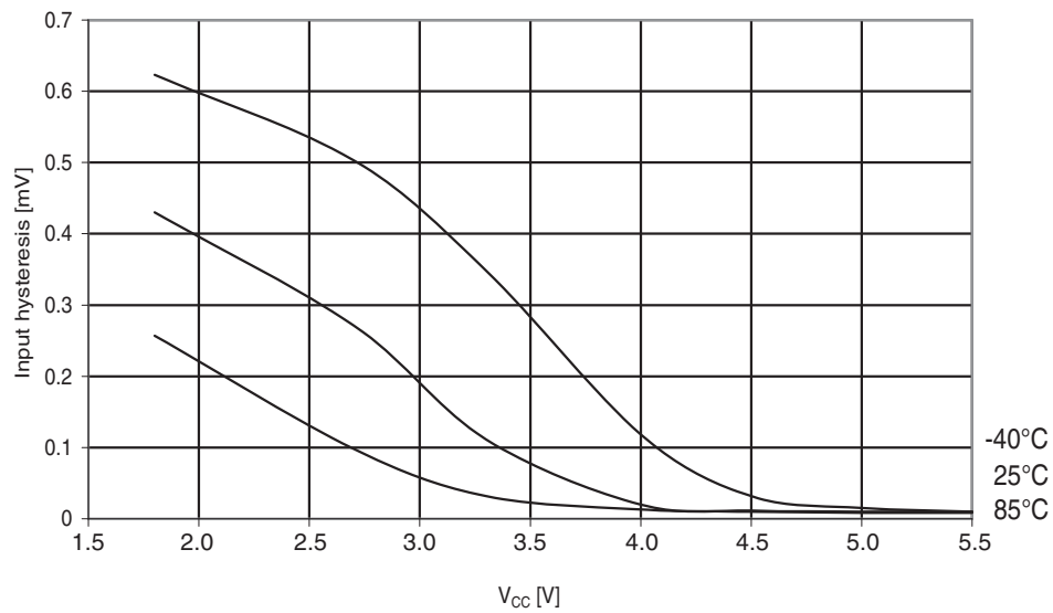
Figure 30-226. ATmega644A: Reset pin input hysteresis vs. V_{CC}
