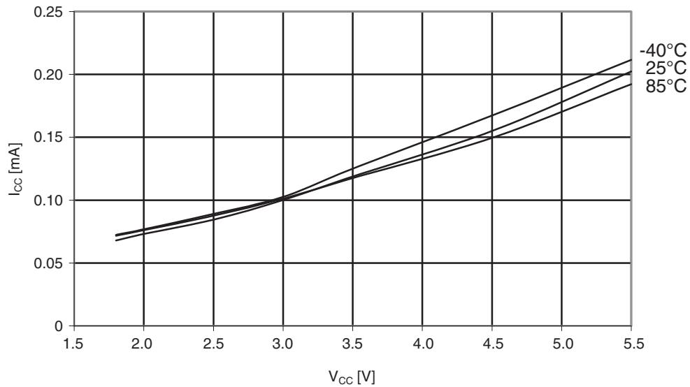
Figure 30-5. ATmega164A: Active supply current vs. V_{CC} (internal RC oscillator, 128kHz)
