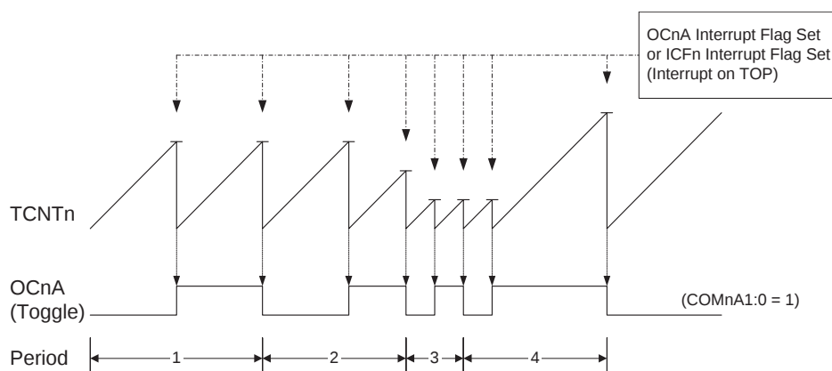
Figure 51. CTC Mode, Timing Diagram
