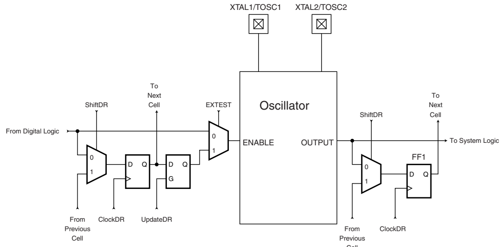
Figure 90. Boundary-scan Cells for Oscillators and Clock Options
