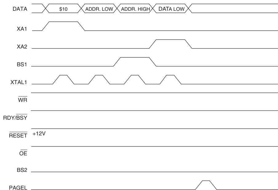
Figure 73. Programming the Flash Waveforms
