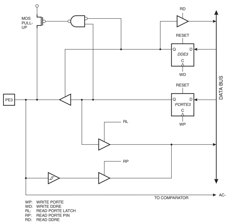
Figure 69. Port E Schematic Diagram (Pin PE3)
