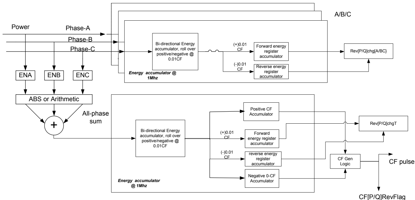
Figure-3 Energy Register Operation Diagram
