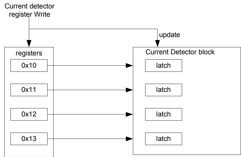
Figure-21 Current Detection Register Latching Scheme
