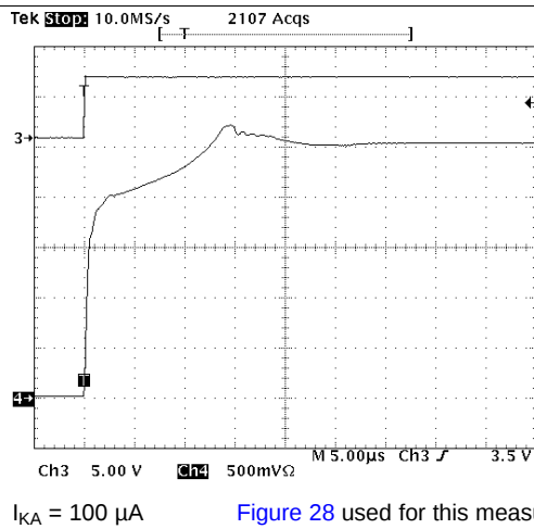
Figure 13. Pulse Response
