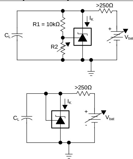
Figure 27. Test Circuit for Stability Boundary Conditions
