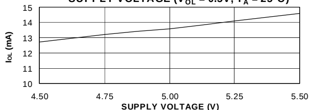
ATF2500C OUTPUT SINK CURRENT VS. SUPPLY VOLTAGE ( V_{OL} = 0.5V , T_A = 25^\circ C )
