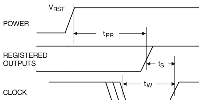
Figure 7-1. Programming/Erasing Timing
