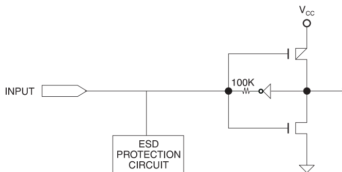
Figure 8-1. Input Diagram
