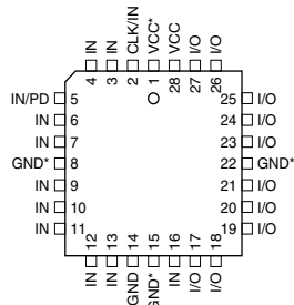
Figure 2-3. PLCC
