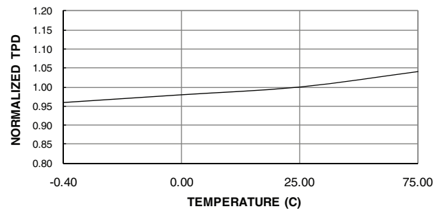
NORMALIZED T_{PD} VS. TEMP
