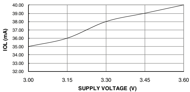
ATMEL ATF22LV10C OUTPUT SINK CURRENT VS. SUPPLY VOLTAGE ( V_{OL} = 0.5\text{V} )
