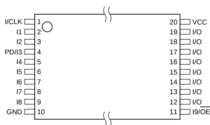
DIP/SOIC
