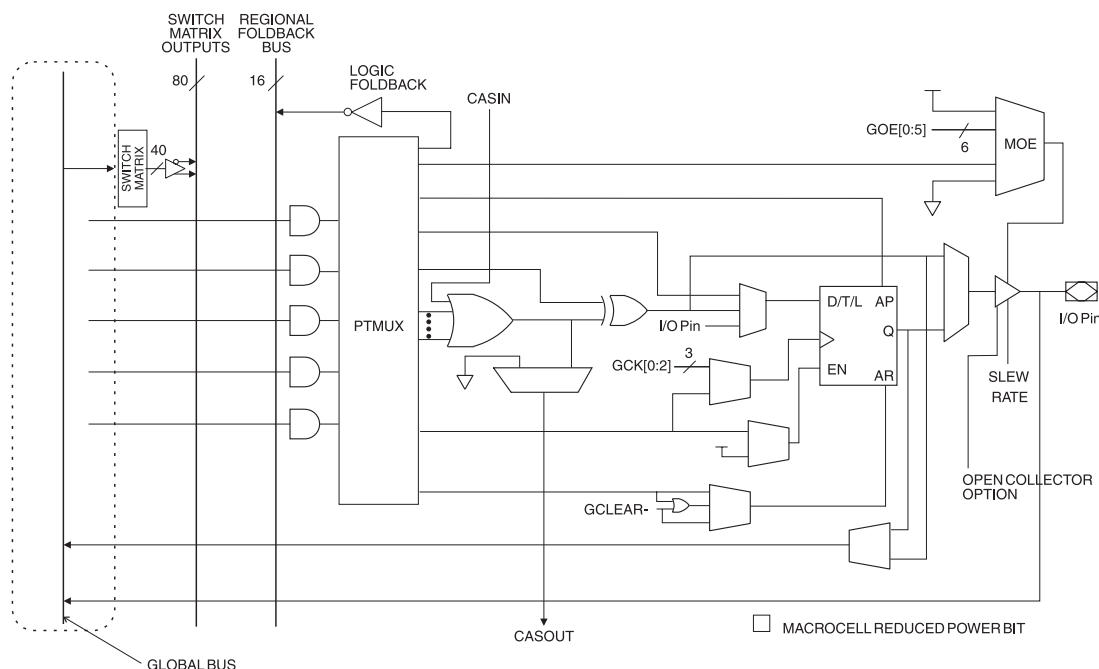
Figure 1. ATF1508AS Macrocell
