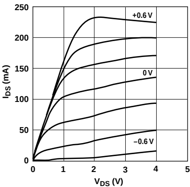
Figure 1. Typical I-V Curves. (V GS = -0.2 V per step)
