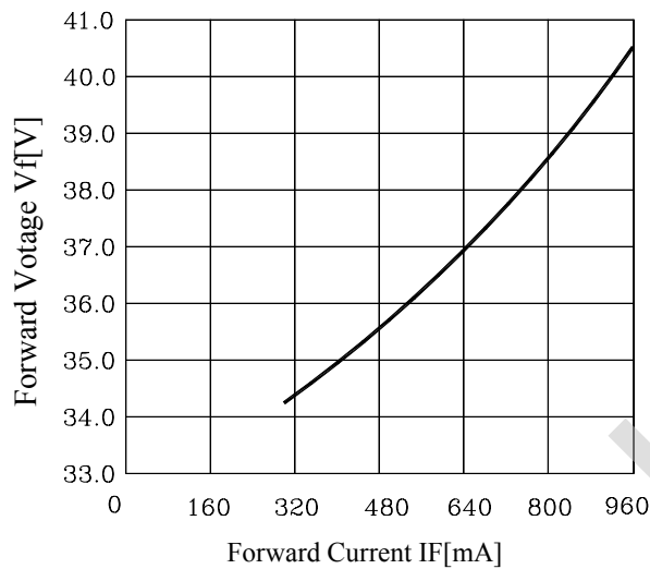
Forward Votage Vs. Forward Current
