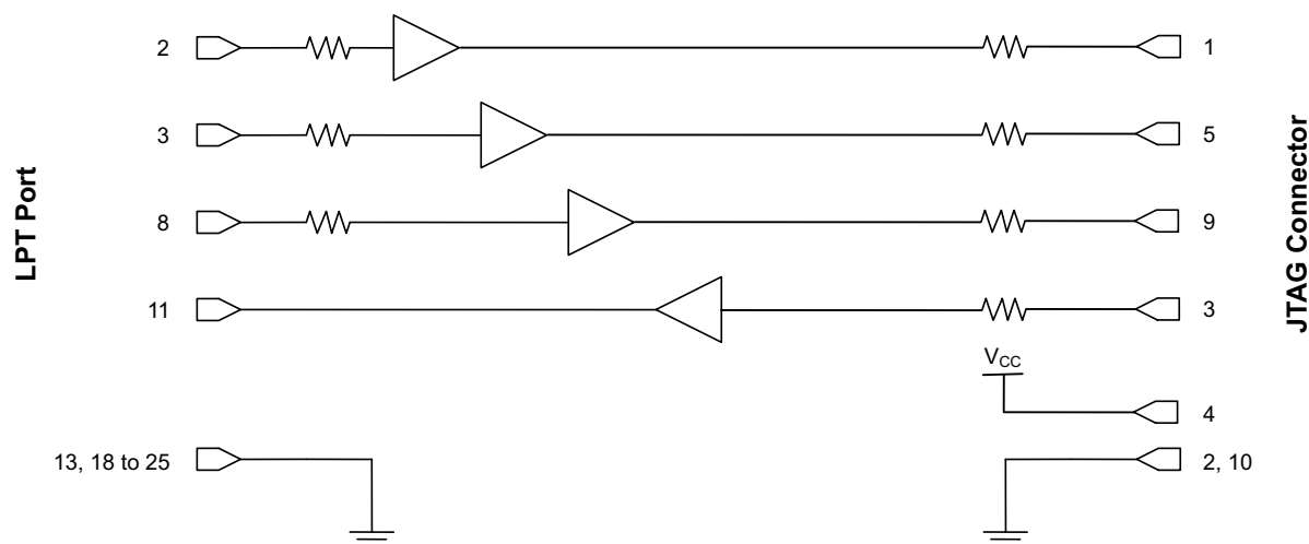
Figure 1. ATF15xx JTAG ISP Download Cable Functional Block Diagram
