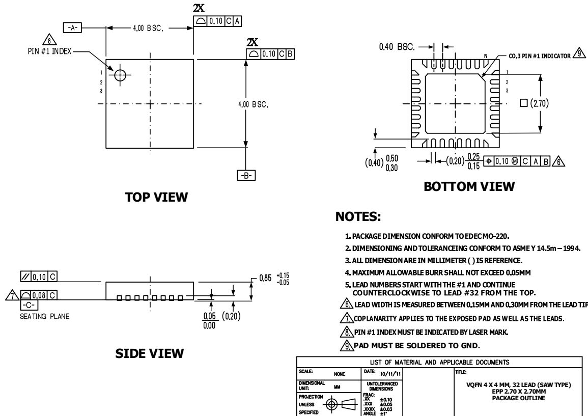
Figure 12-1. ATBTLC1000 4x4 QFN 32 Package Outline Drawing
