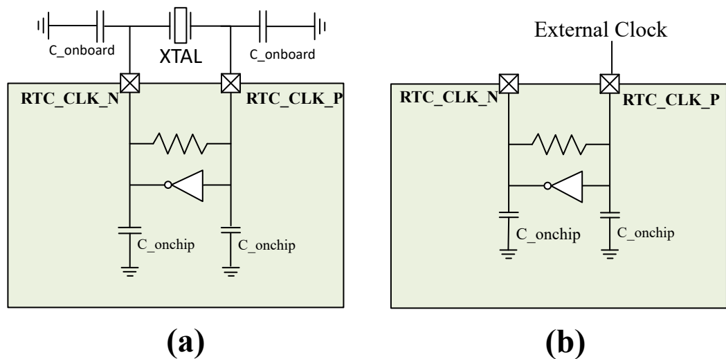
Figure 7-3. ATBTLC1000 Connections to RTC XO
