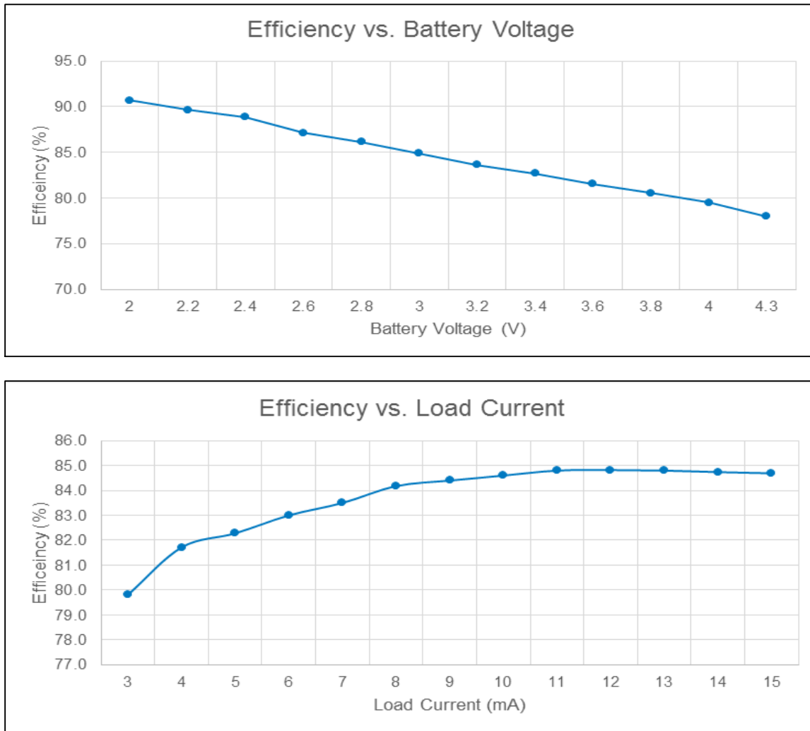
Figure 6-2. DC/DC Converter Efficiency
