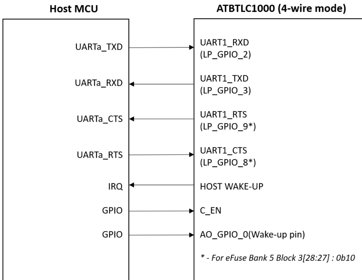
Figure 5-1. Host Microcontroller to ATBTLC1000-QFN Interface - 4-Wire Mode
