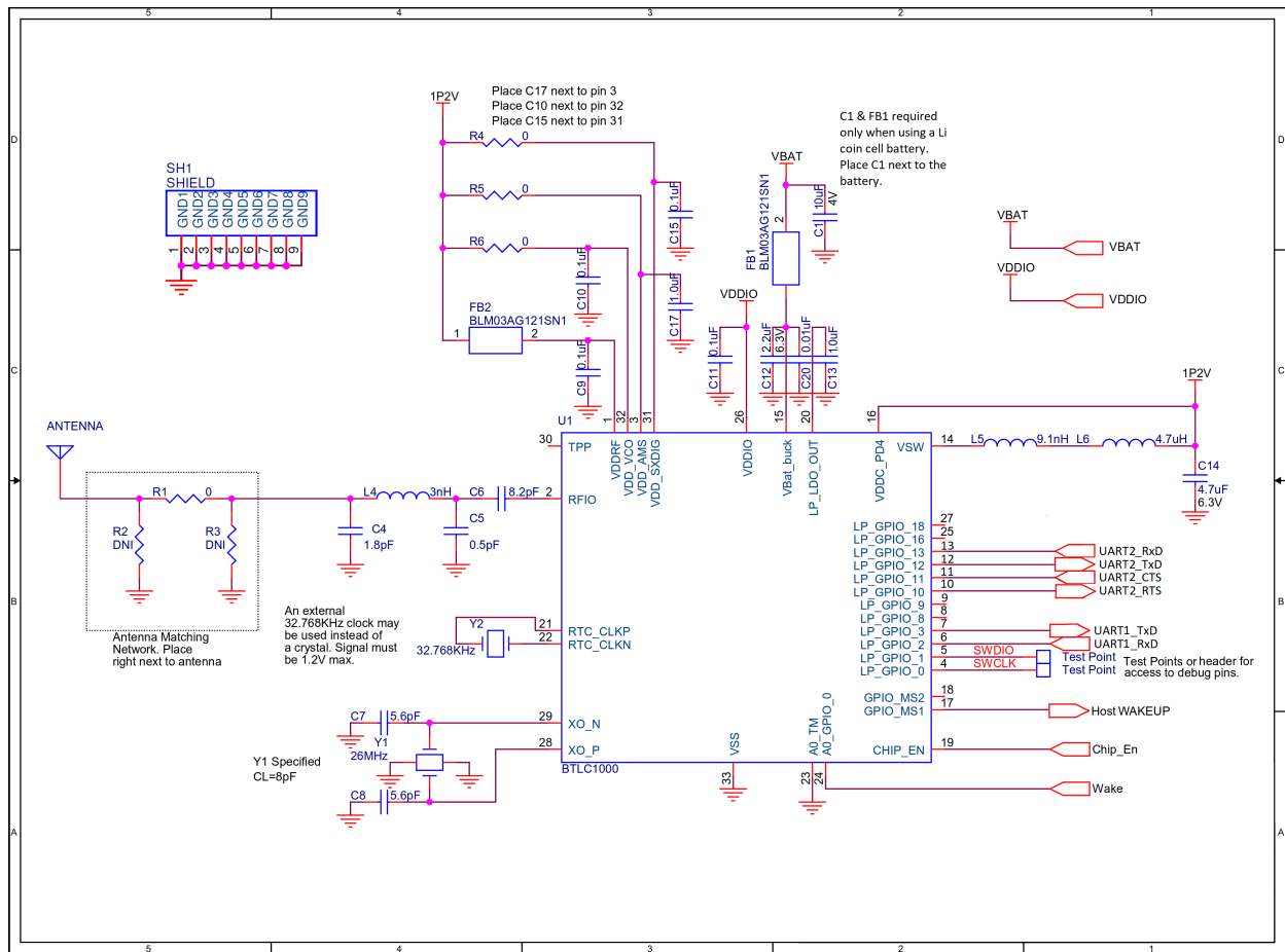
Figure 13-2. ATBTLC1000 QFN Reference Design (6-wire)
