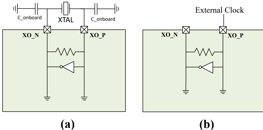
Figure 7-2. ATBTLC1000 Connections to XO
