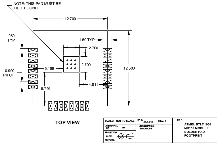
Figure 9-2. Customer PCB Footprint
