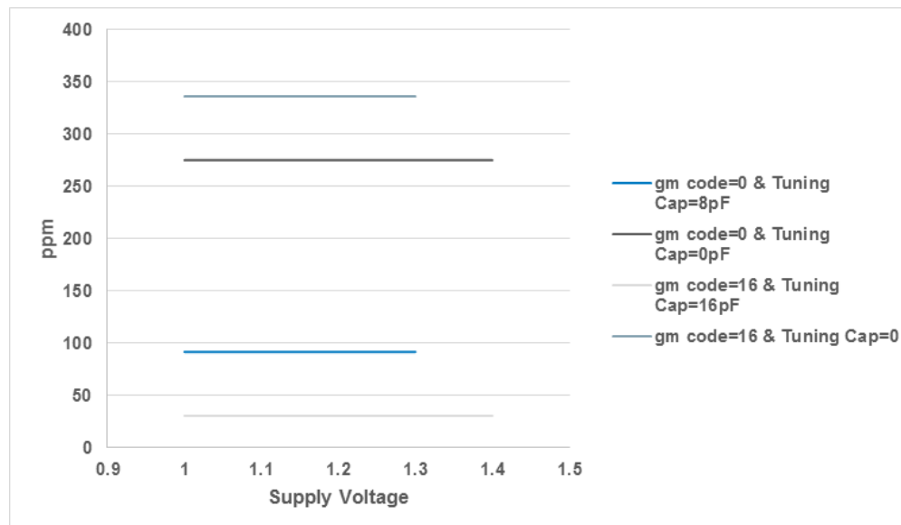
Figure 7-6. RTC Frequency Deviation vs. Supply Voltage
