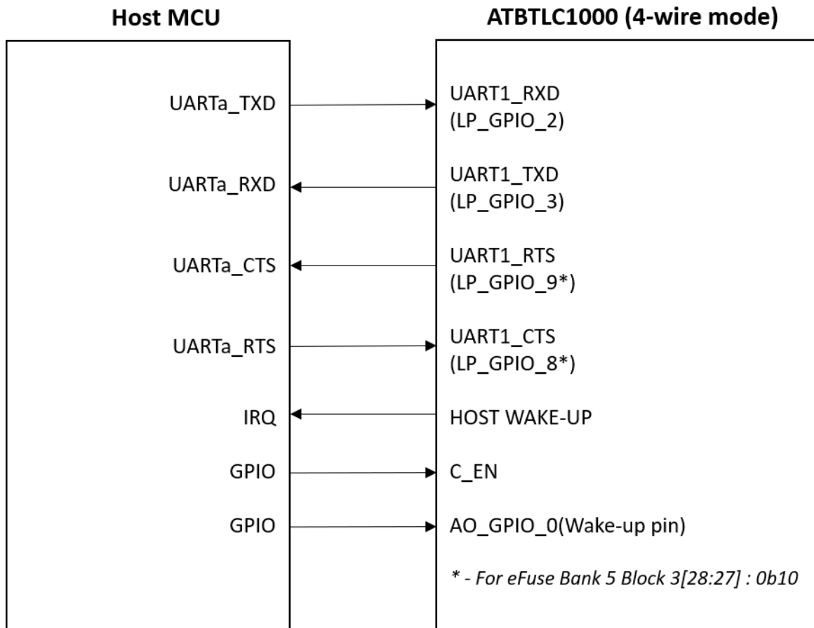
Figure 6-1. Host Microcontroller to ATBTLC1000-MR110CA Interface - 4-wire Mode
