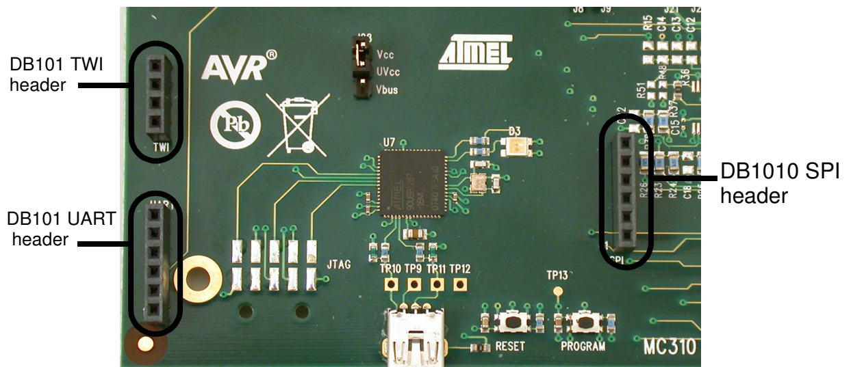
Figure 2-5. DB101 headers
