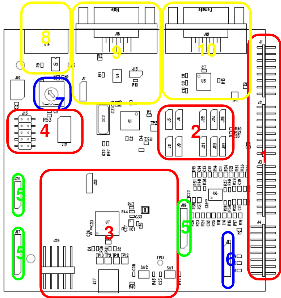
Figure 2-1. MC310 PCB layout
