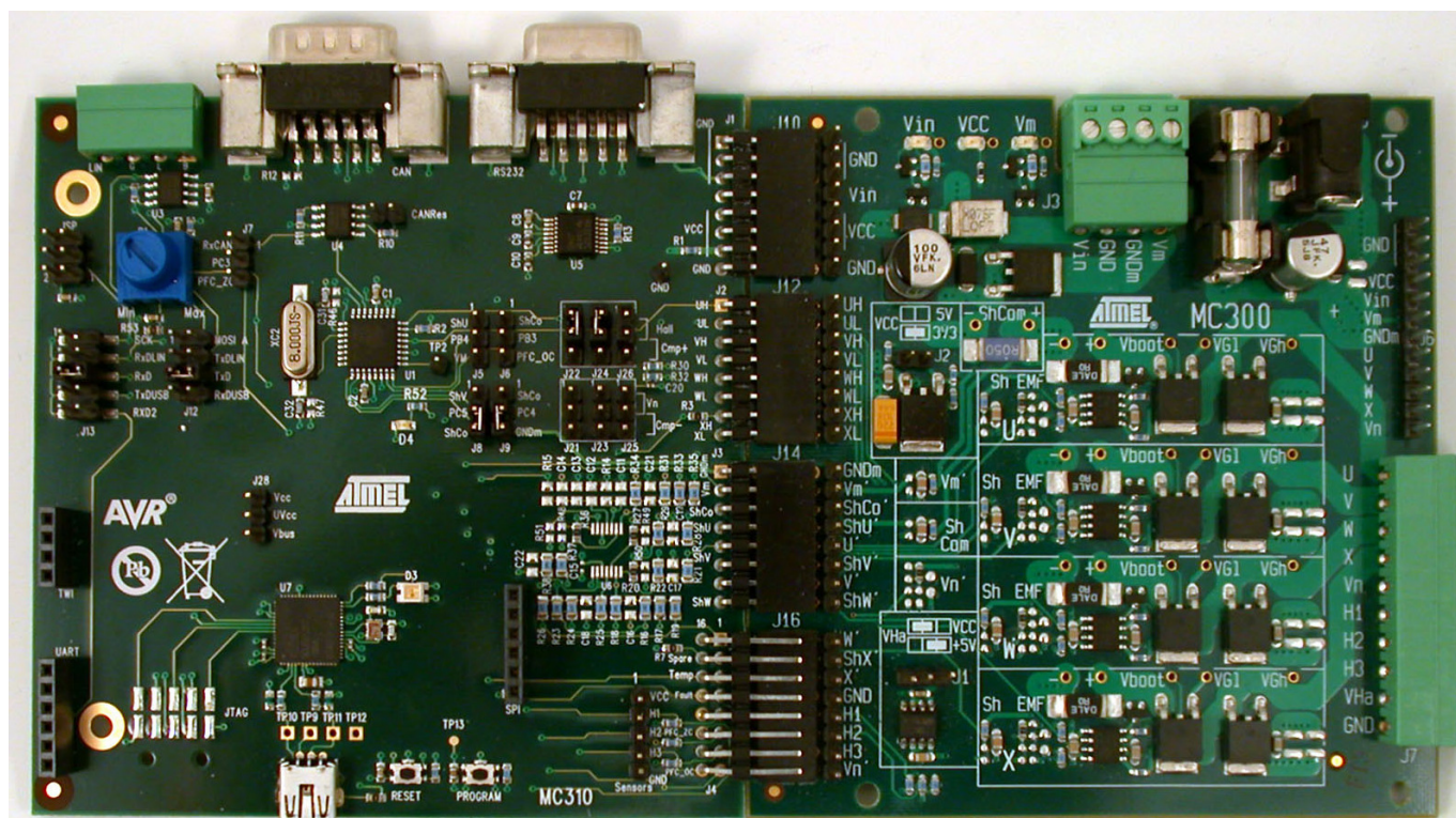
Figure 2-2. MC310 device board with power board MC300
