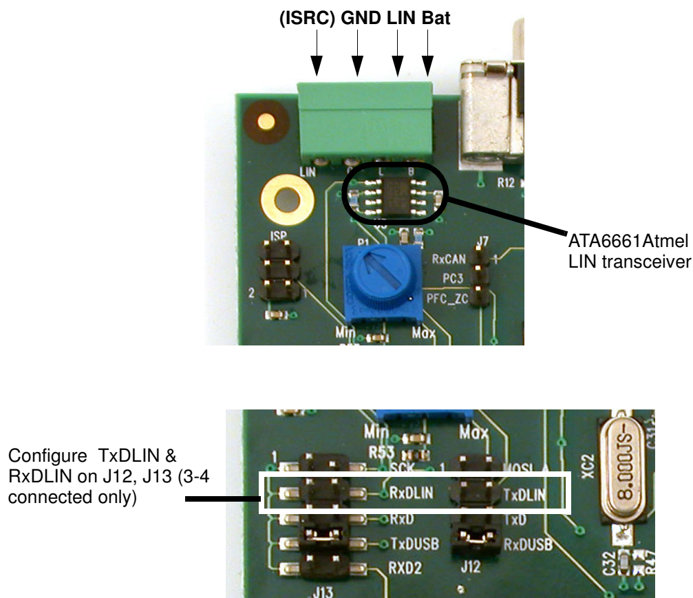
Figure 2-6. LIN connector
