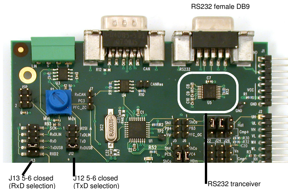
Figure 2-9. RS232 connector & configuration
