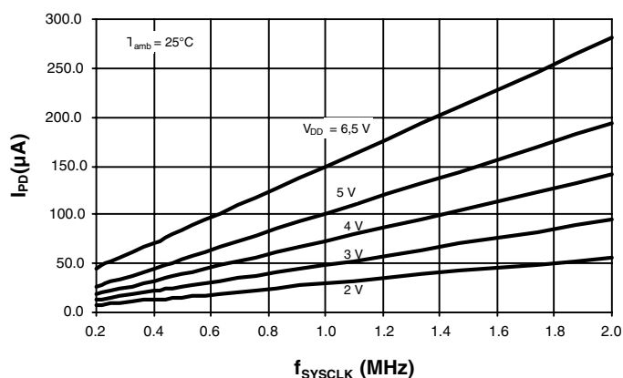
Figure 60. Power-down Supply Current versus Frequency
