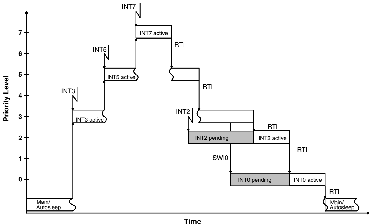
Figure 8. Interrupt Handling
