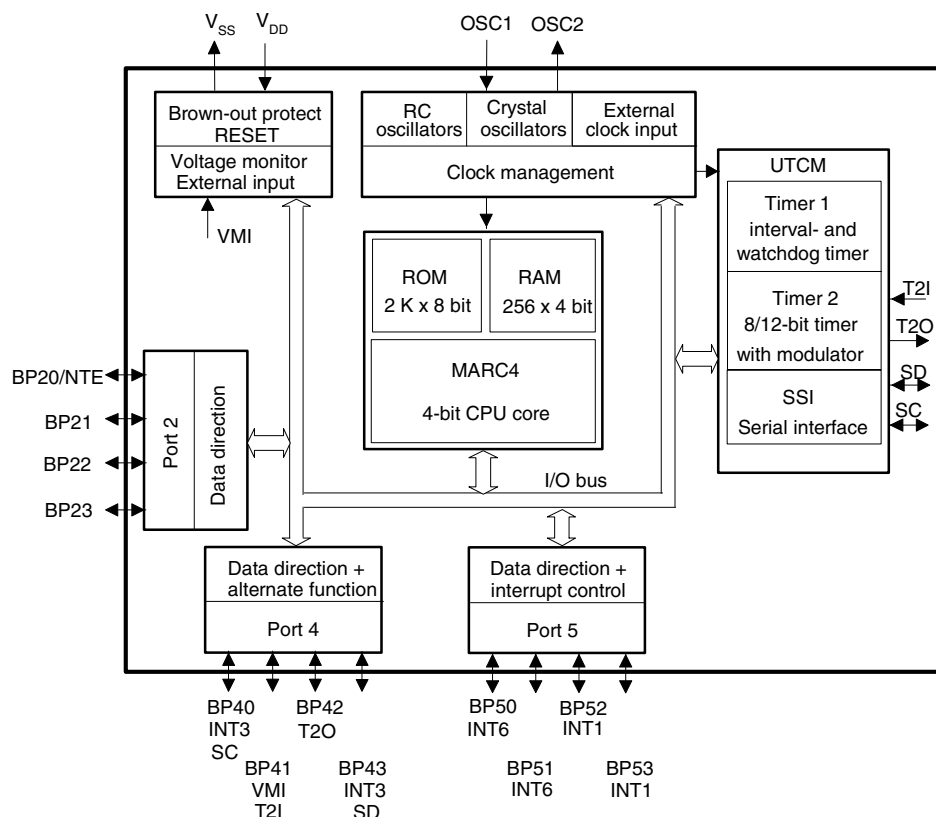
Figure 1. Block Diagram
