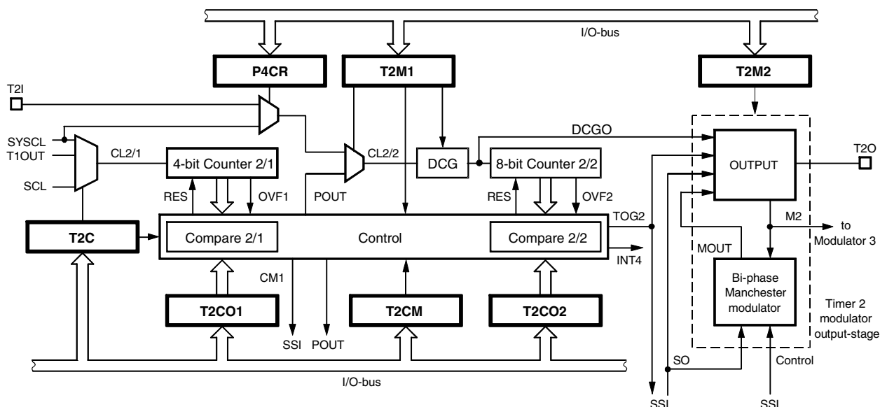
Figure 29. Timer 2
