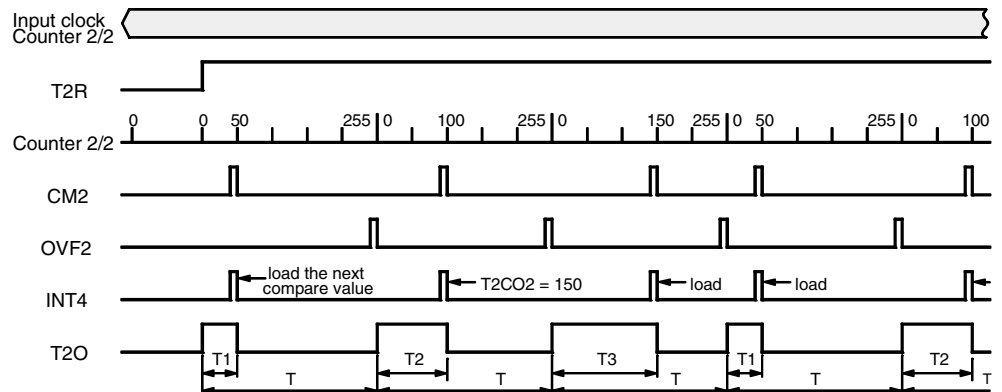
Figure 41. PWM Modulation
