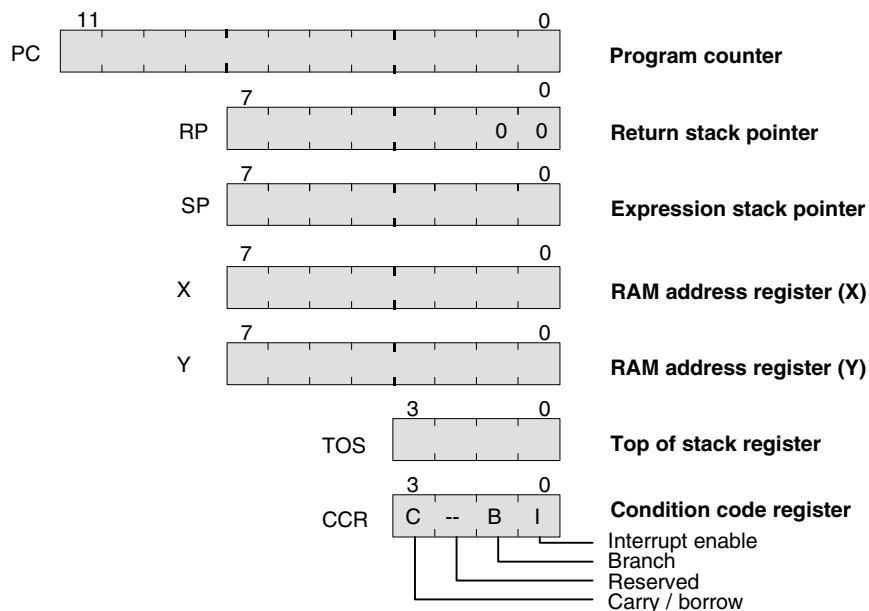
Figure 6. Programming Model
