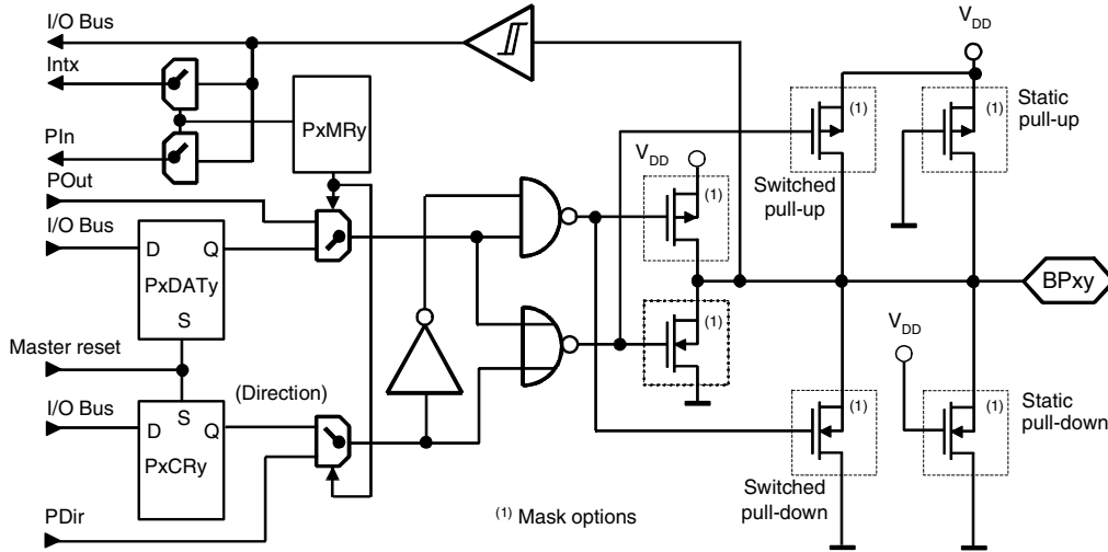
Figure 25. Bi-directional Port 4 and Port 6
