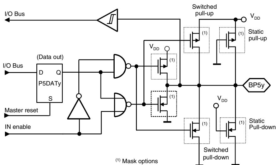
Figure 23. Bi-directional Port 5
