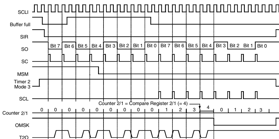
Figure 56. Manchester Modulation 2
