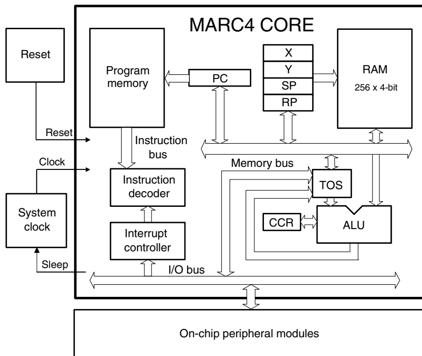
Figure 3. MARC4 Core
