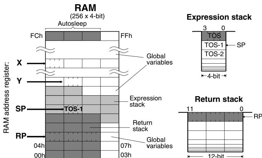
Figure 5. RAM Map
