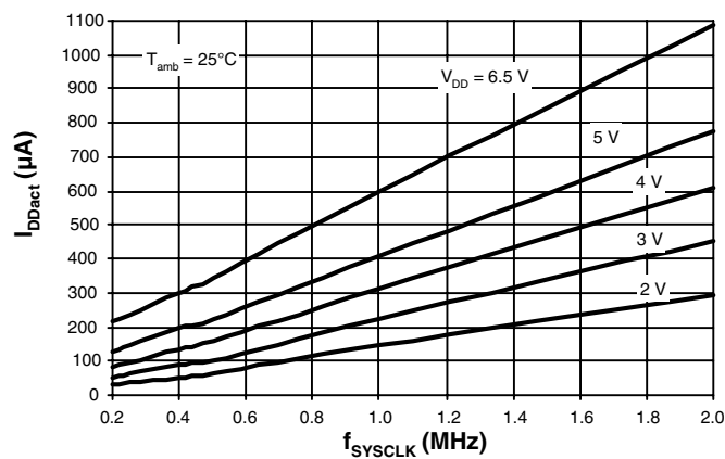
Figure 59. Active Supply Current versus Frequency
