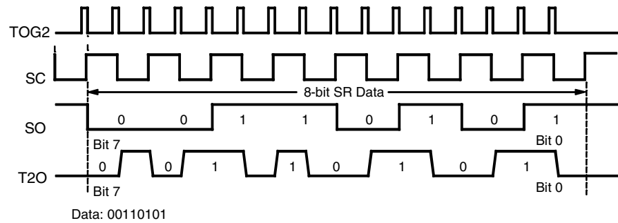
Figure 40. Manchester Modulation
