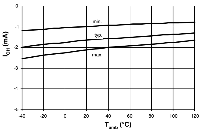
Figure 80. Output High Current versus T_{amb} , V_{DD} = 2\text{ V} , V_{OH} = 0.8 \times V_{DD}
