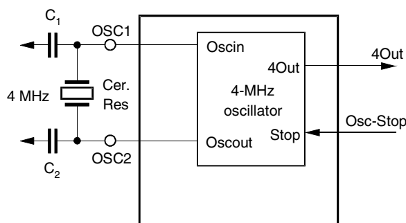
Figure 19. Ceramic Resonator
