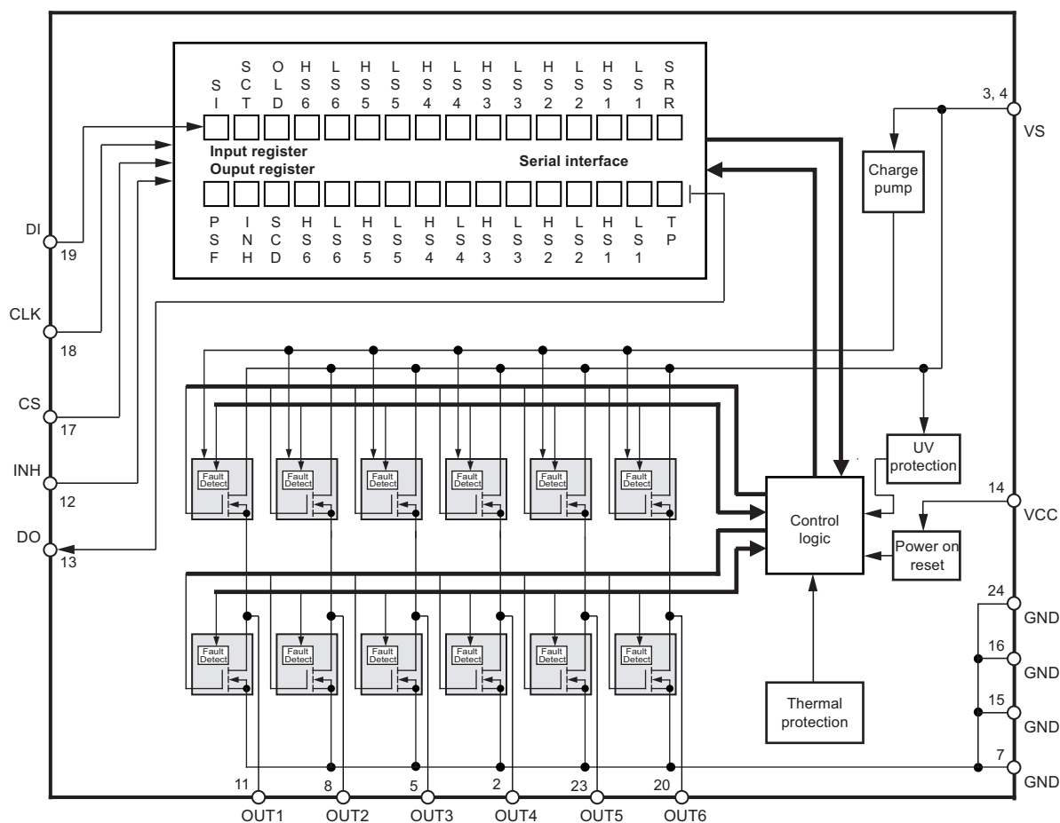
Figure 1-1. Block Diagram QFN24
