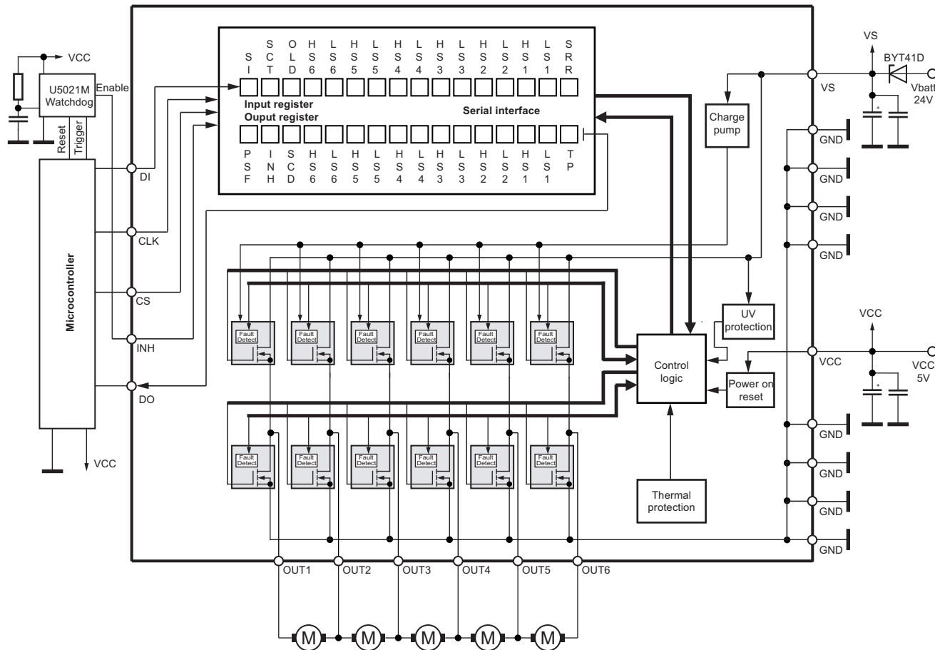
Figure 10-1. Application Circuit
