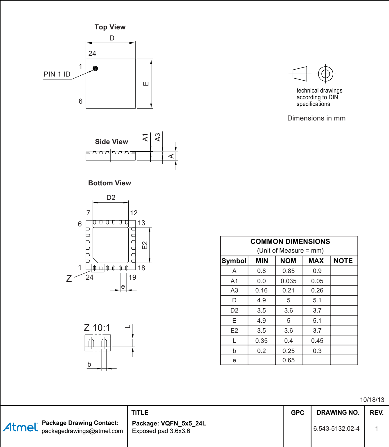
Figure 12-2. QFN24
