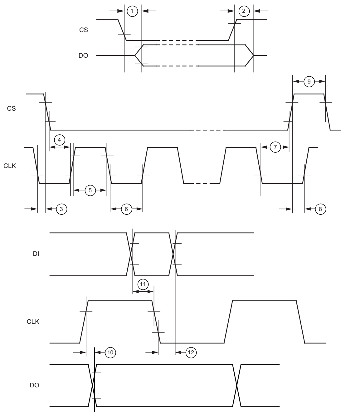
Figure 9-1. Serial Interface Timing with Chart Number
