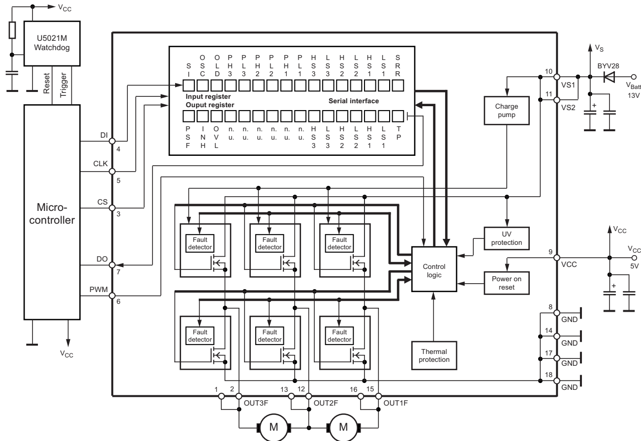
Figure 10-1. Application Circuit
