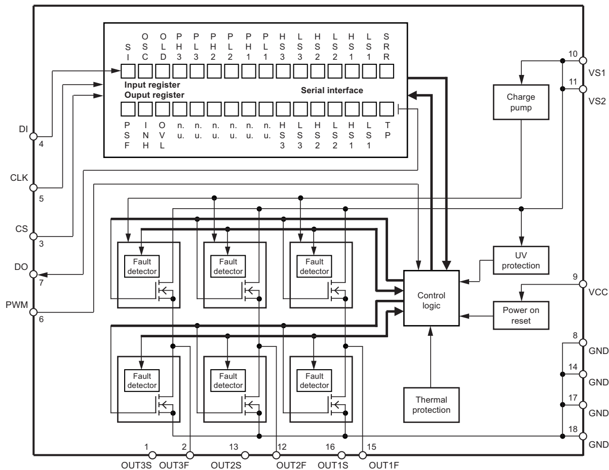
Figure 1-1. Block Diagram
