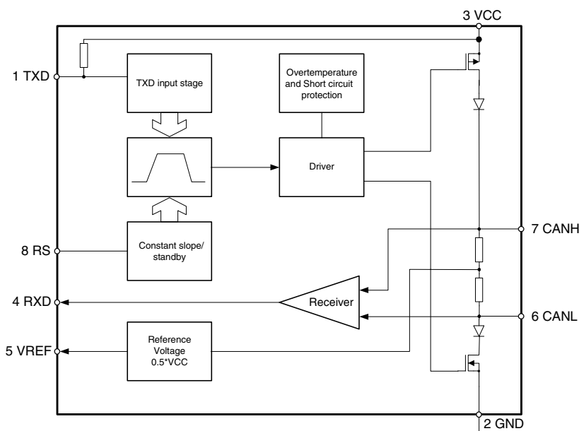
Figure 1. Block Diagram
