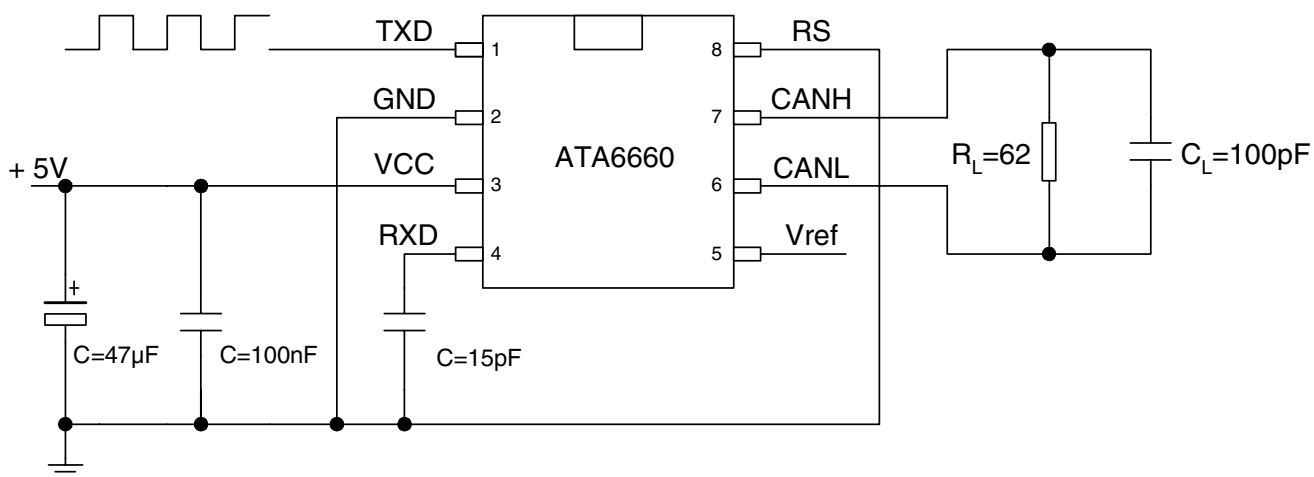
Figure 4. Test Circuit for Timing Characteristics
