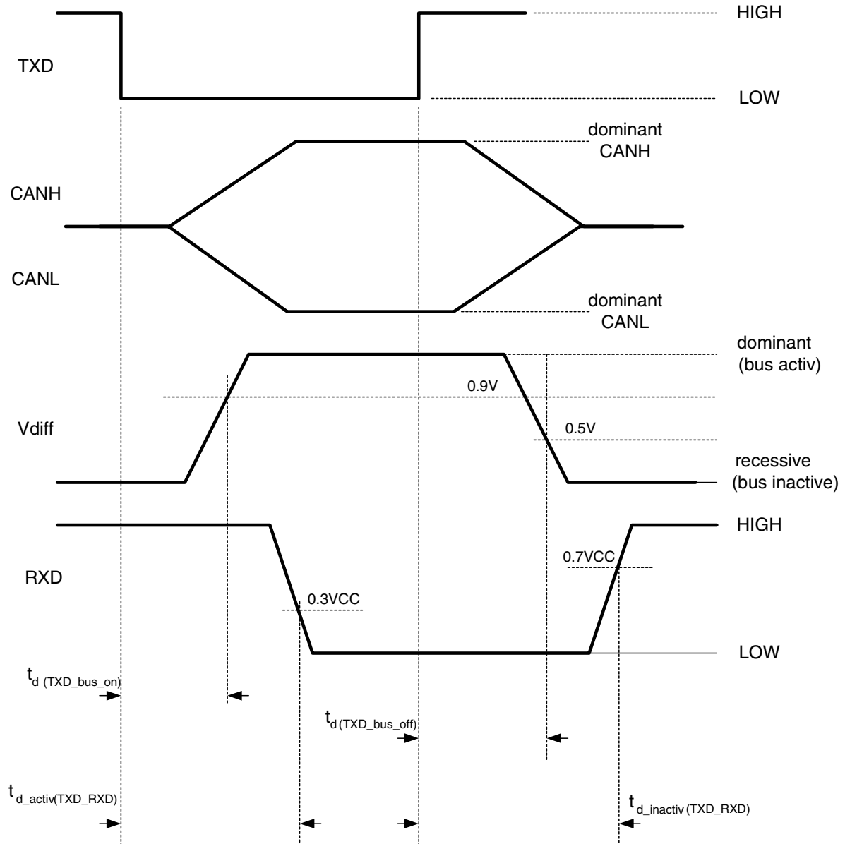
Figure 3. Timing Diagrams
