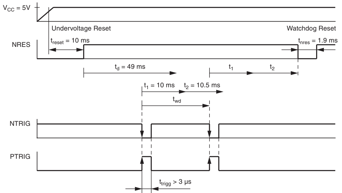
Figure 3-8. Timing Sequence with R_{\text{WD\_OSC}} = 51 k \Omega
