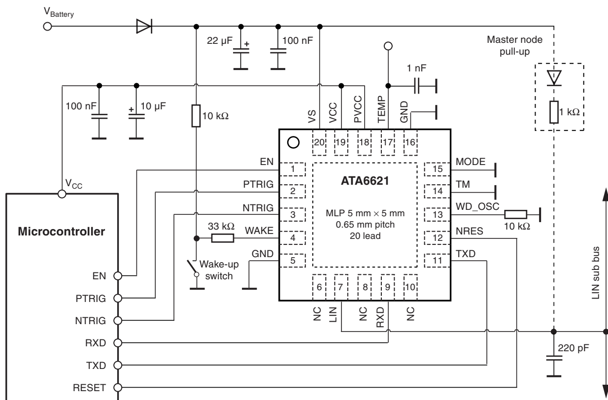
Figure 5-2. Application Circuit
