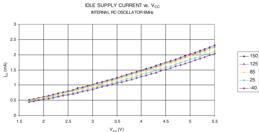
Figure 4-120. Idle Supply Current versus V_{CC} (Internal RC Oscillator, 8MHz)
