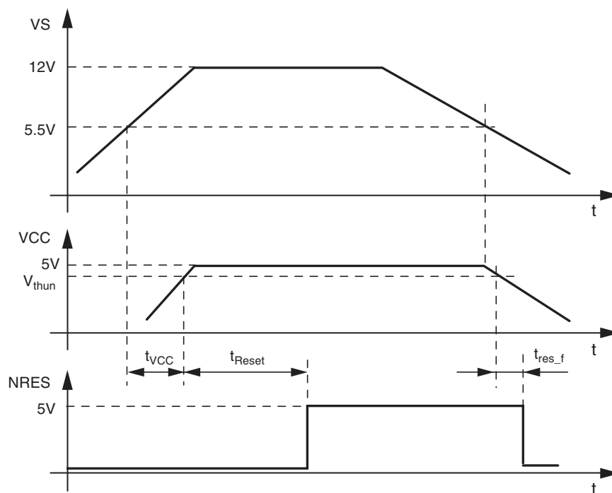
Figure 3-7. VCC Voltage Regulator: Ramp-up and Undervoltage Detection
