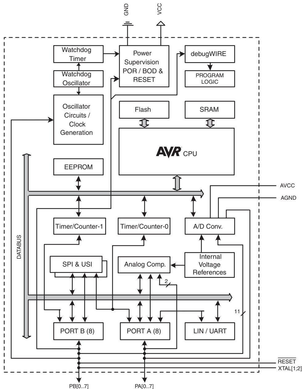
Figure 4-1. Block Diagram
