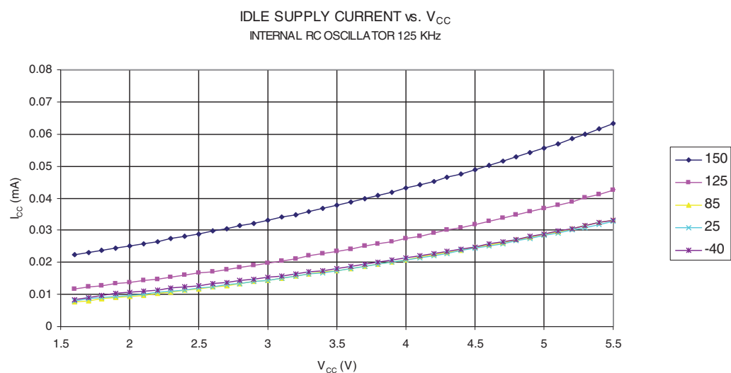
Figure 4-121. Idle Supply Current versus 5V_{CC} (Internal RC Oscillator, 128kHz)
