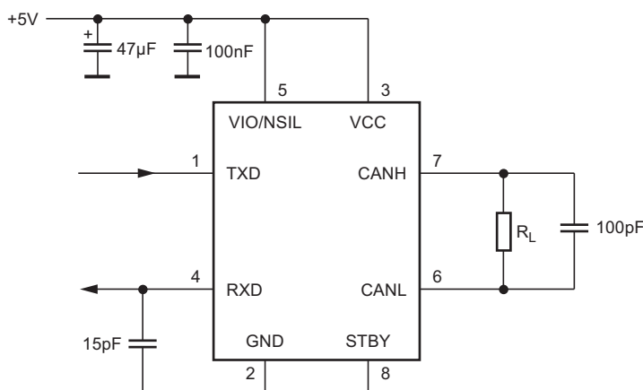
Figure 5-1. Test Setup for Timing Measurements
