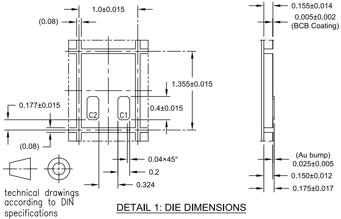
Figure 9-3. Sawn Wafer on Foil with Ring (Gold Bumps)
