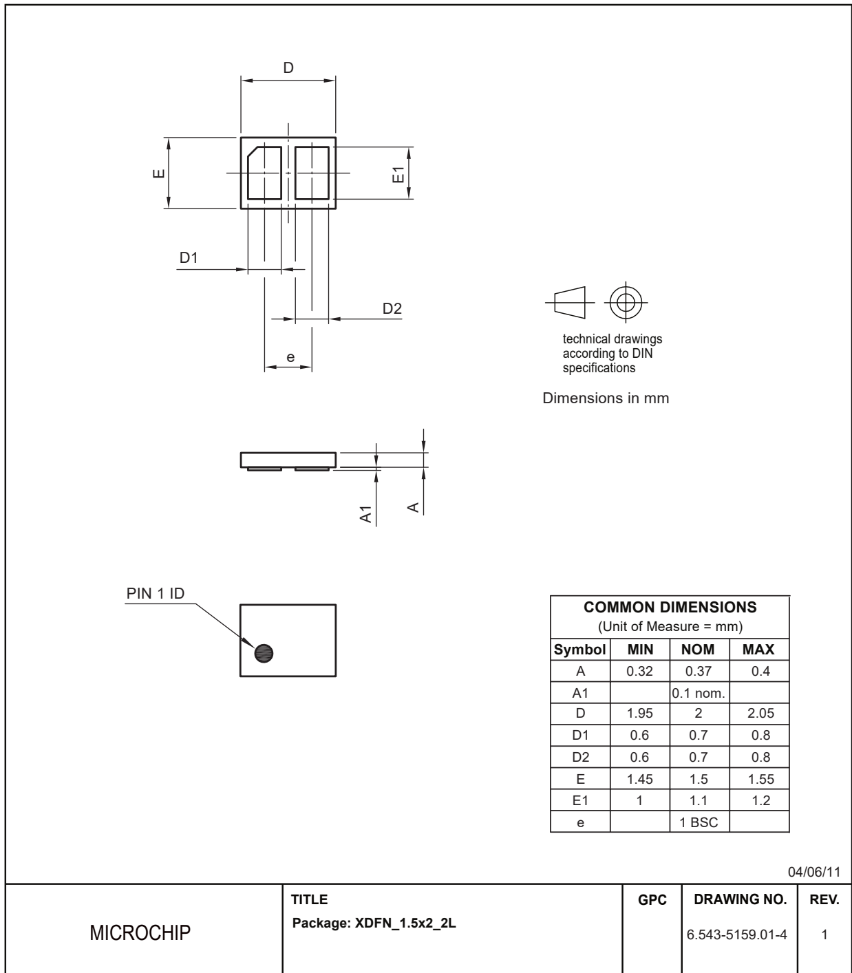
Figure 9-7. XDFN Package
