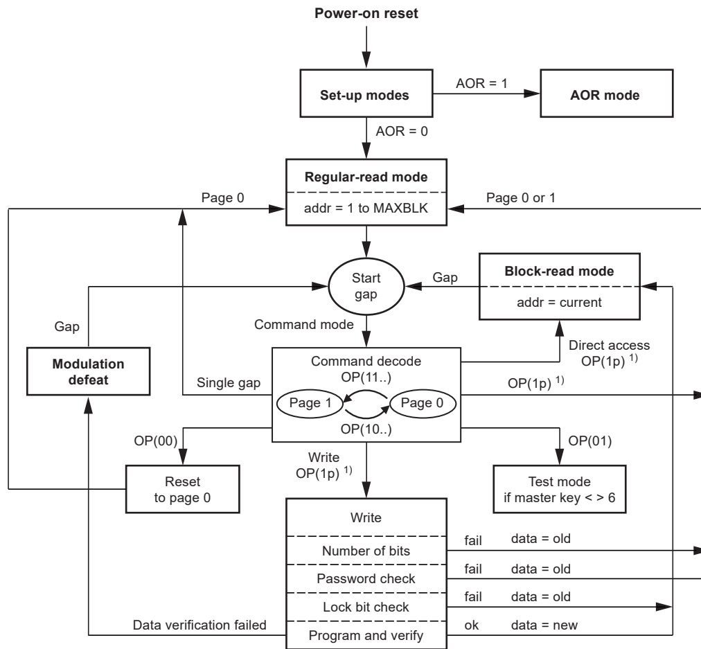
Figure 5-1. ATA5577C Functional Diagram
