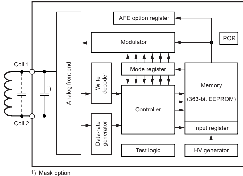
Figure 3-1. Block Diagram
