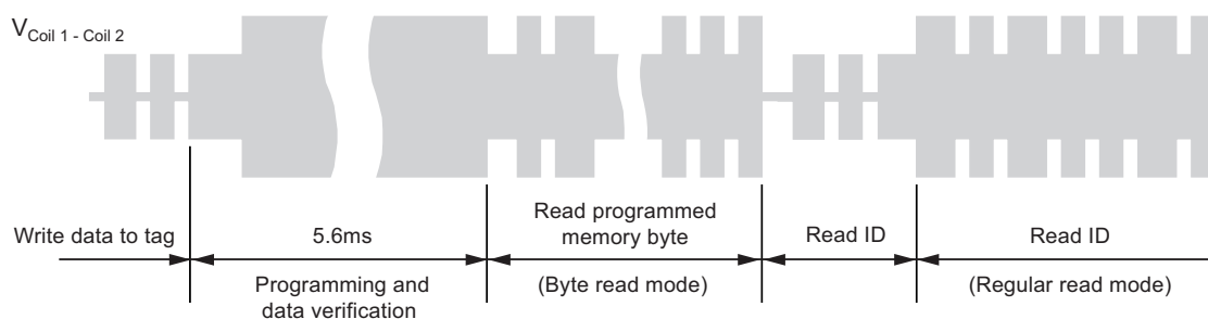
Figure 5-5. Coil Voltage after Programming a Byte
