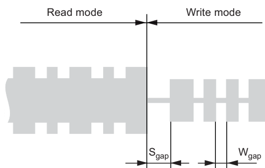
Figure 5-2. Start of Reader-to-tag Communication (Downlink)
