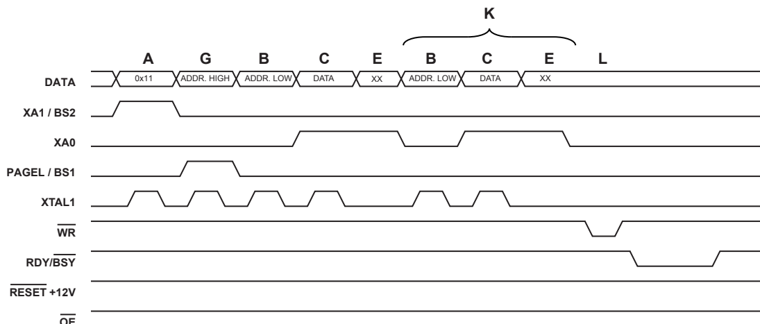
Figure 22-4. Programming the EEPROM Waveforms
