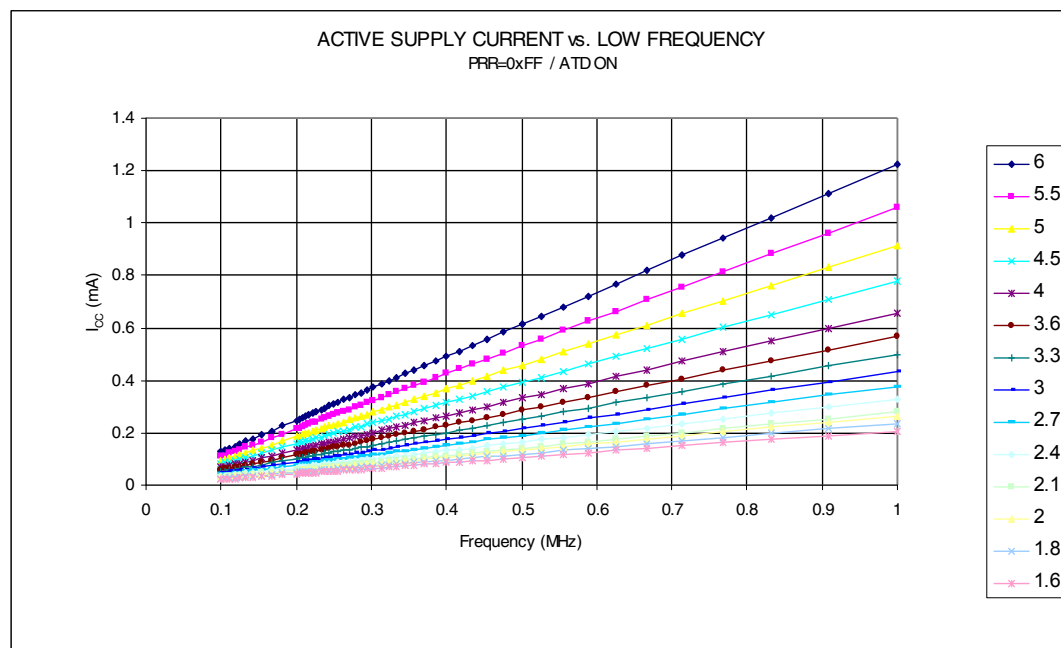
Figure 25-1. Active Supply Current versus Low Frequency (0.1 - 1.0MHz)
