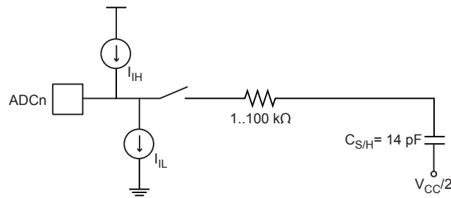
Figure 18-8. Analog Input Circuitry
