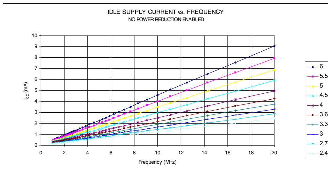
Figure 25-5. Idle Supply Current vs. Frequency ( \geq 1 MHz)
