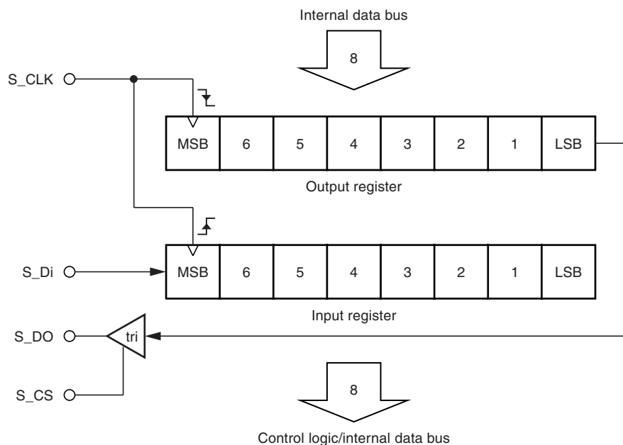
Figure 3-6. SPI Structure
