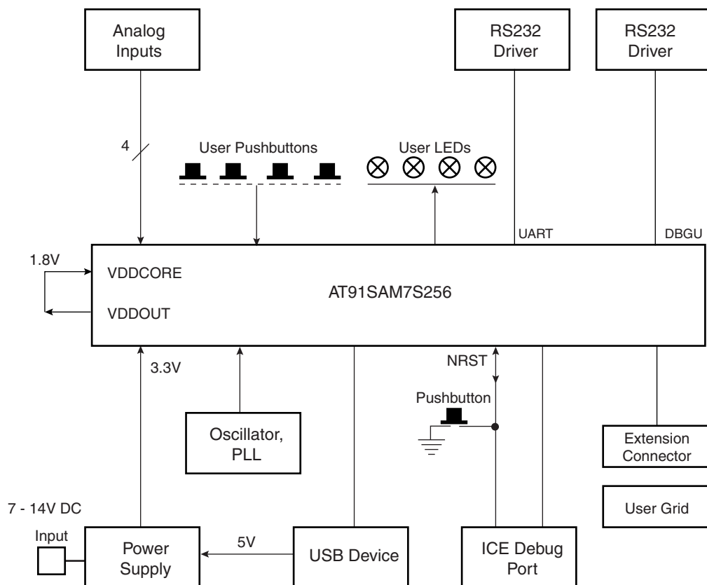
Figure 2-1. Block Diagram for AT91SAM7S-EK Board
