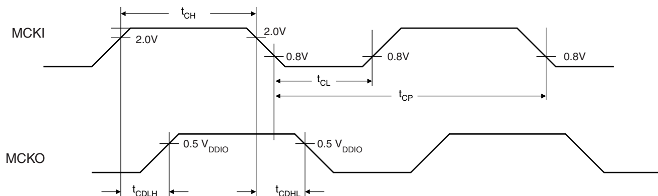
Figure 6-1. Clock Waveform
