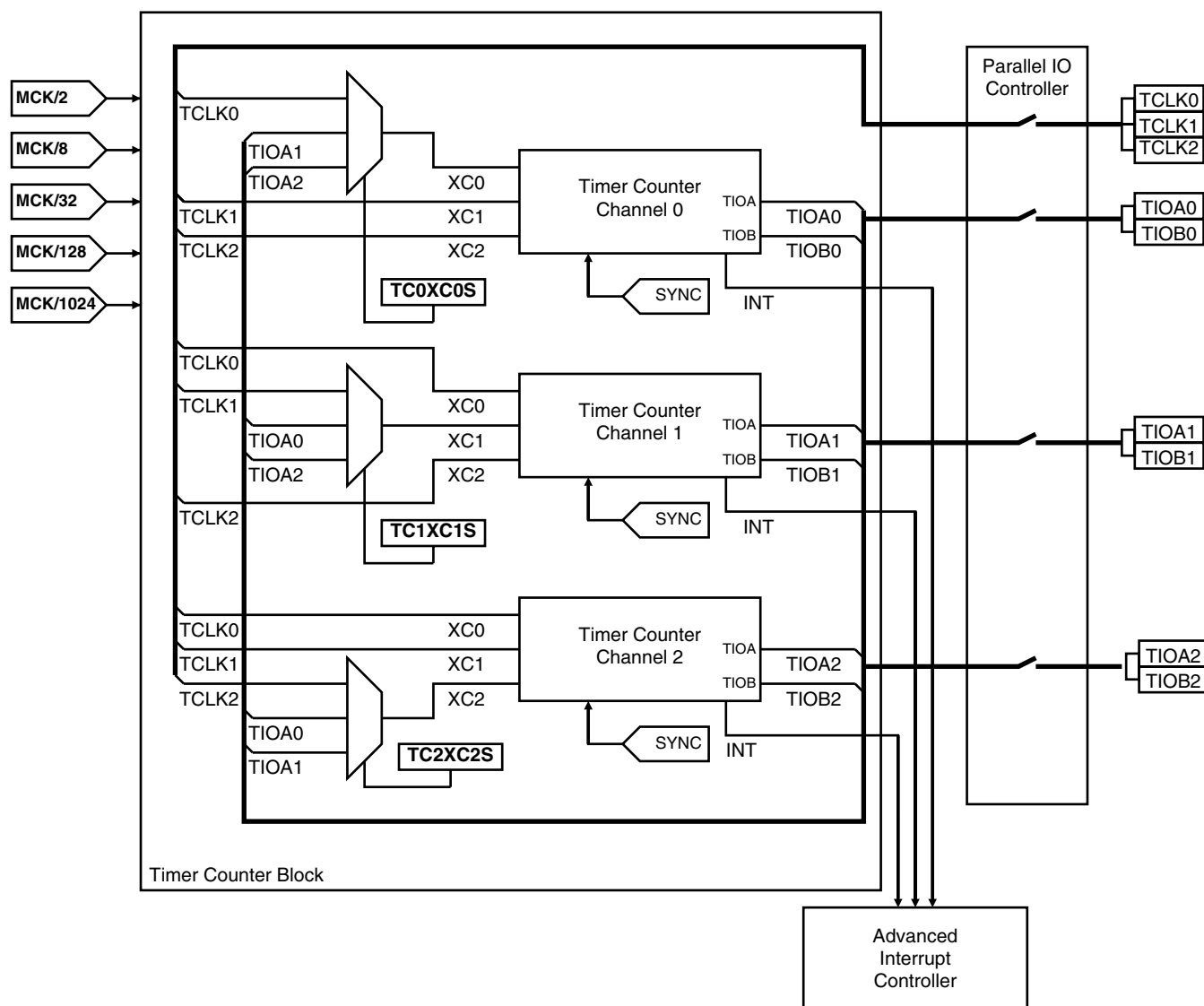
Figure 19-1. TC Block Diagram
