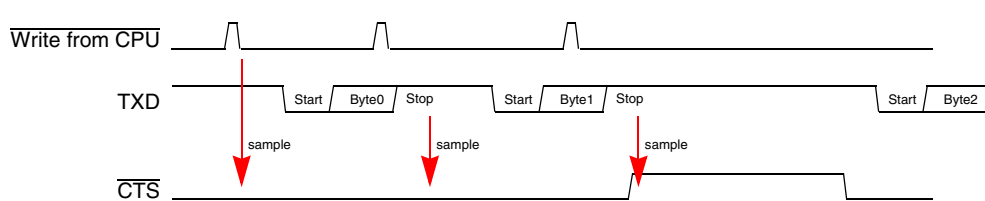
Figure 17-10. \overline{\text{CTS}} behavior
