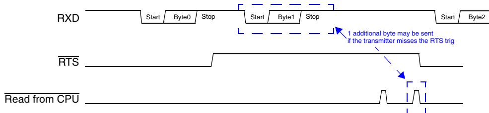
Figure 17-9. \overline{\text{RTS}} behavior
